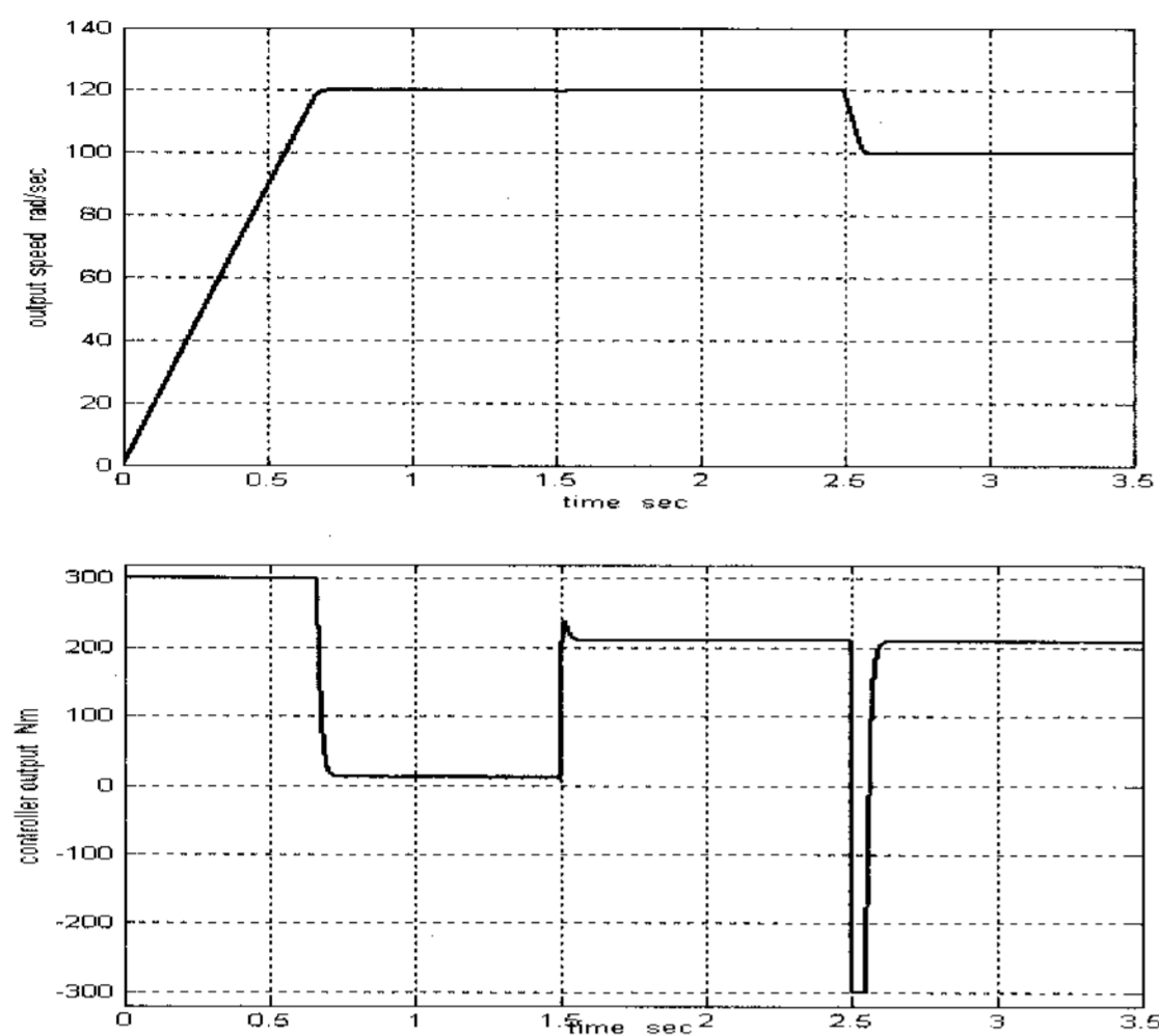
Fig. 13 CSC performance at different operating conditions
