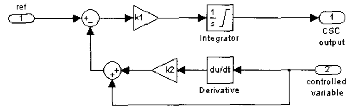
Fig. 2 CSC model in s-domain
