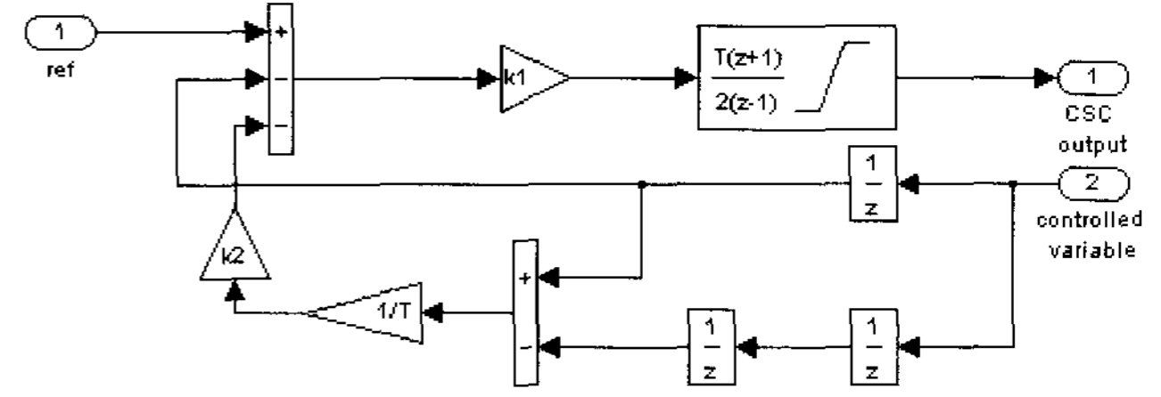
Fig. 1 CSC model in z-domain
