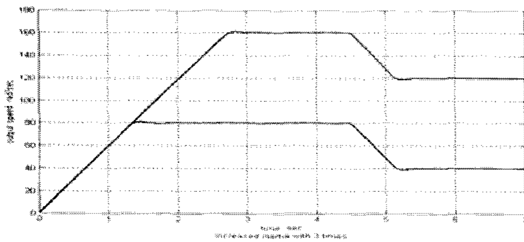
Fig. 10 Responses to a step change of reference speed followed by a step reduction with different inertias
