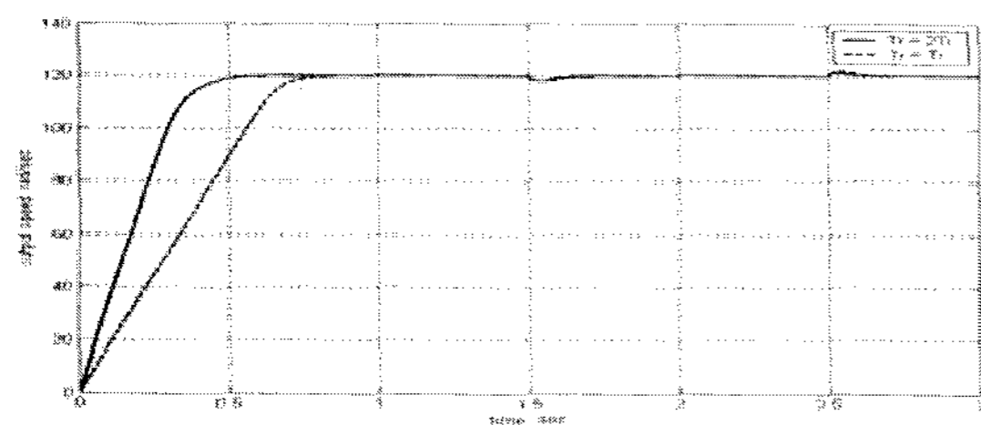
Fig. 11 responses with rotor resistance variations
