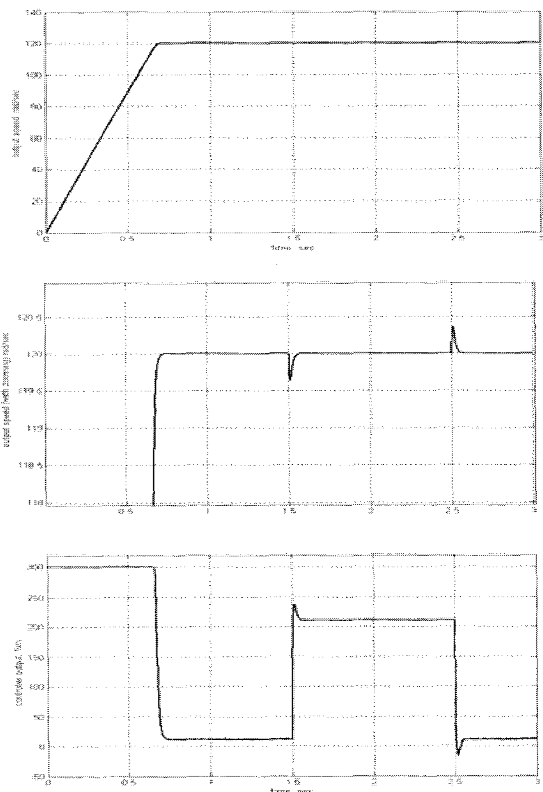
Fig. 12 CSC performance to provide a critically damped speed response and a maximum full load disturbance dip of 0.5rad/sec
