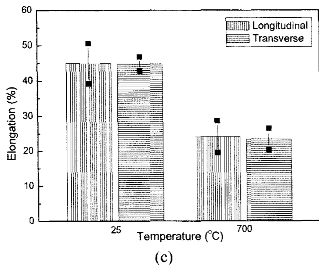
Fig. 7. Tensile Test Results for the Longitudinal and Transverse Directions of the Recrystallization Heat-Treated Austenitic ODS Steels at Room Temperature and at 700°C
