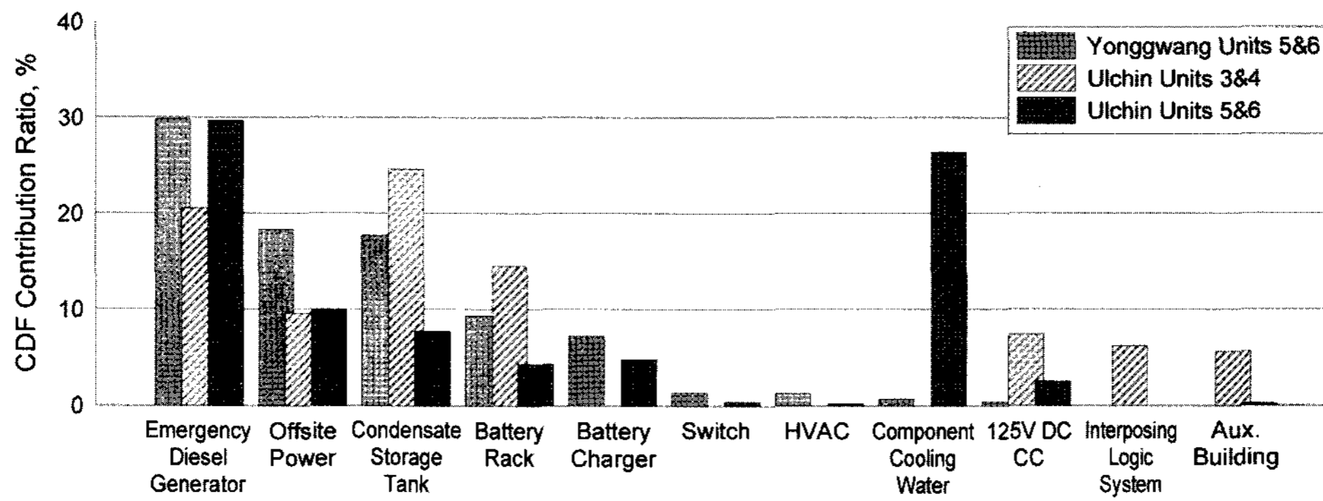
Fig. 18. CDF Contribution Ratios of the Major Equipment and Components at Korean NPPs
