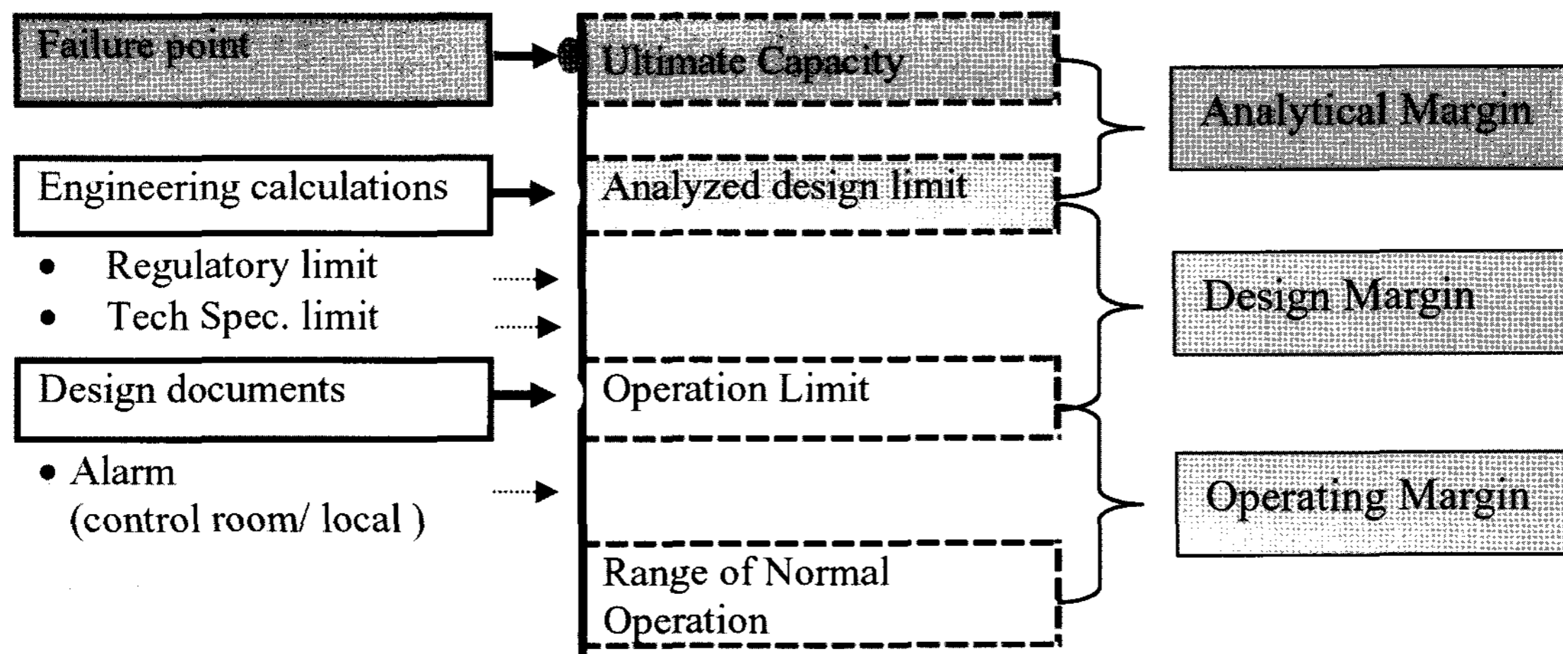
Fig. 3. Design and Operating Margin
