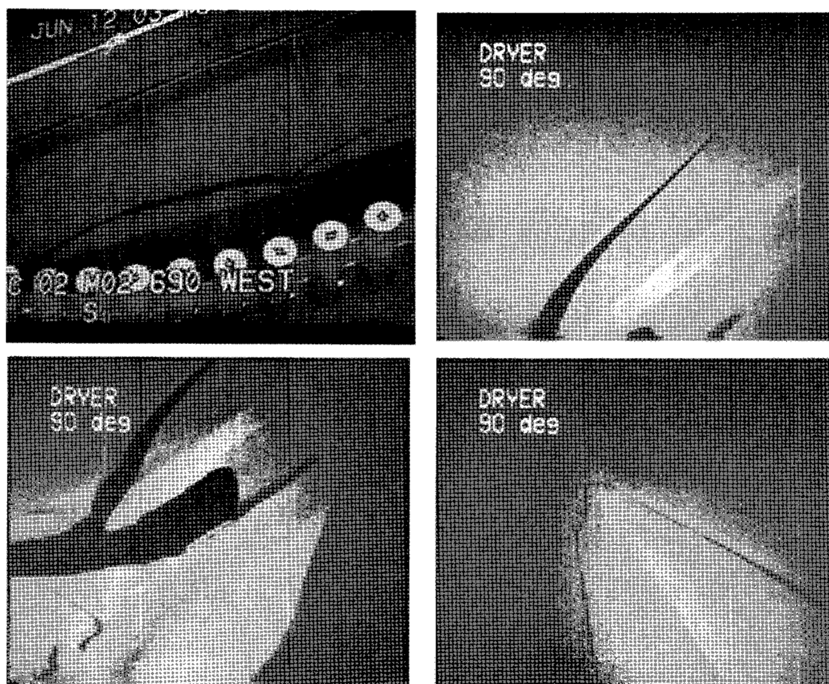
Fig. 4. Steam Dryer Broken in Quad Cities Unit 2
