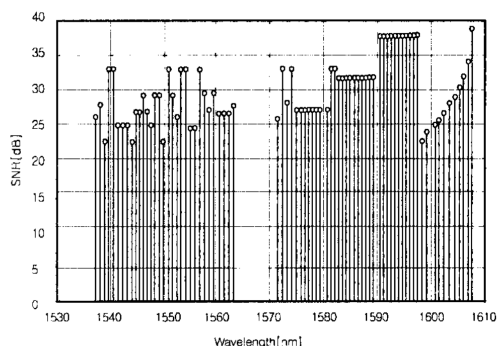
Fig. 9. The SNR of signals from node 21 pre-EDFA
