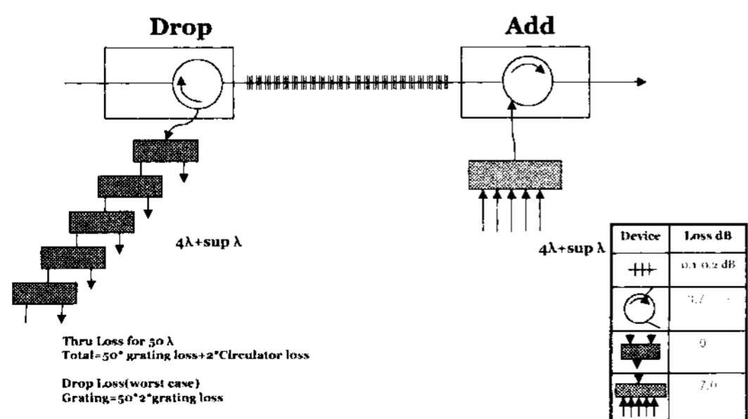
Fig. 2. The fixed add/drop method
