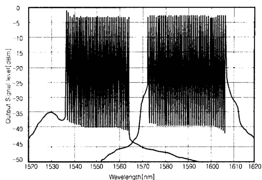
Fig. 8. The output spectra of node 21 pre-EDFA
