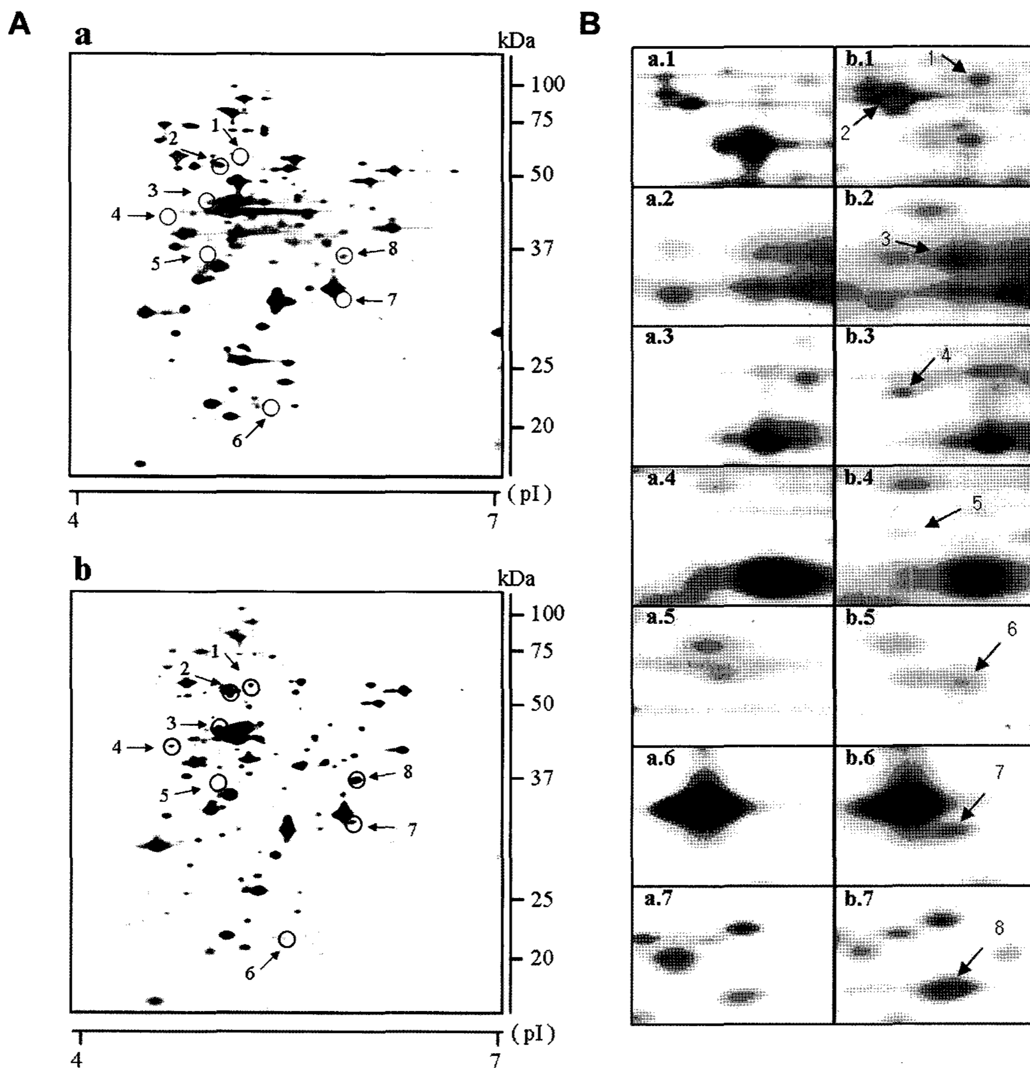
Fig. 1. 2-DE protein profiles of V. vulnificus M06-24/O.
