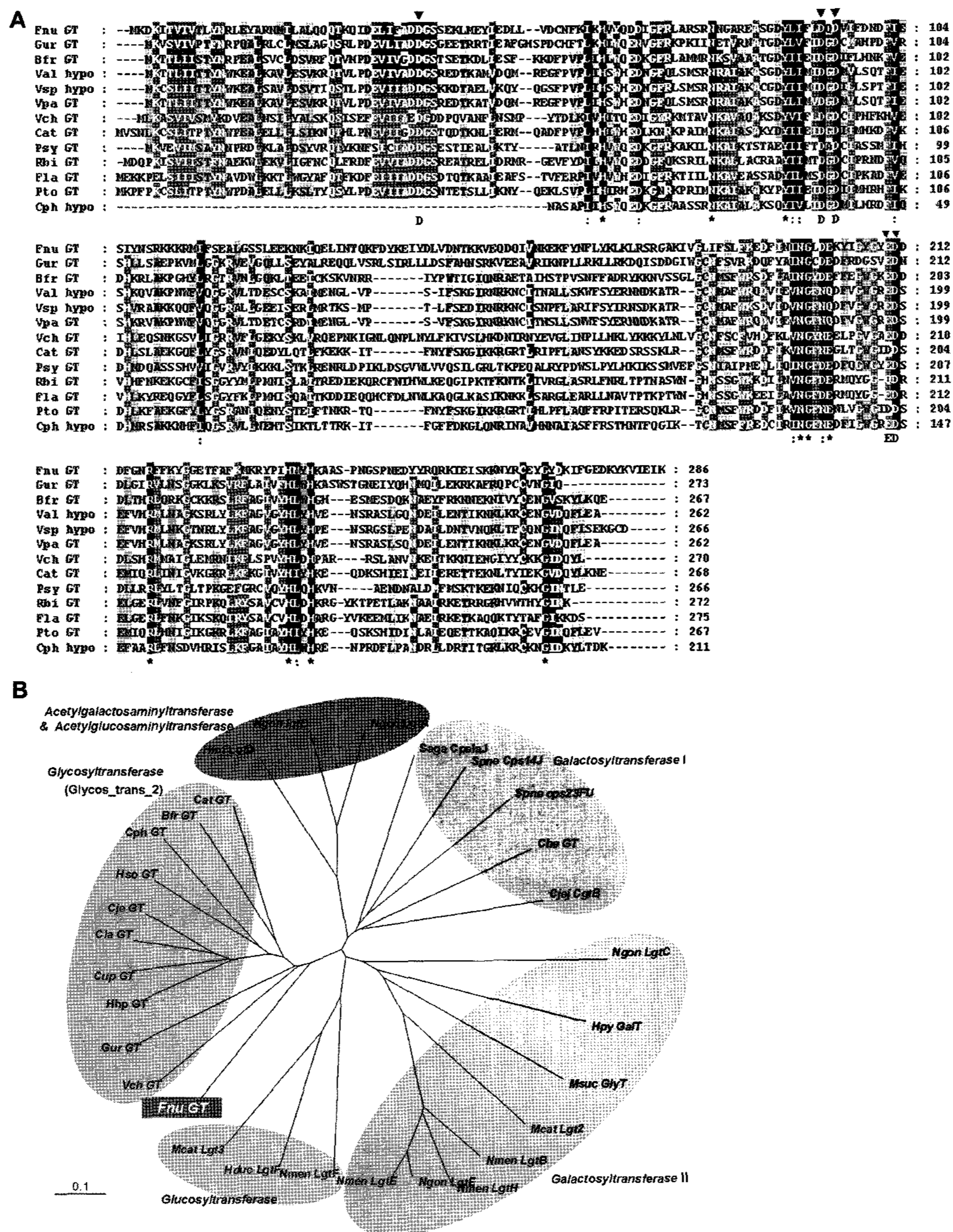
Fig. 1. Bioinformatic analysis of Fnu_GT.
