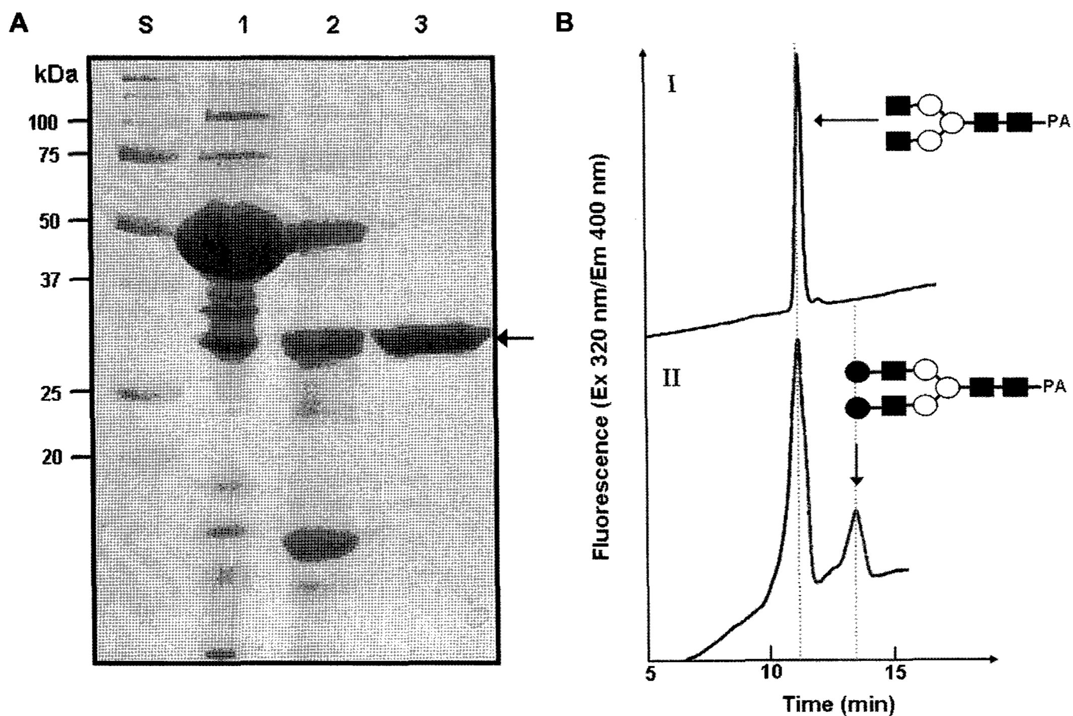
Fig. 2. Purification and galactosyltransferase activity assay of rFnu_GT.
