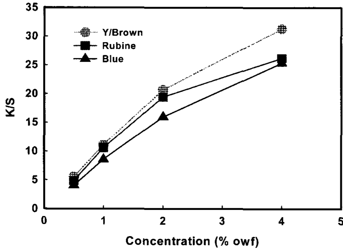
Fig. 2. Build-up properties of PET dyed with S type disperse dye at 120°C.
