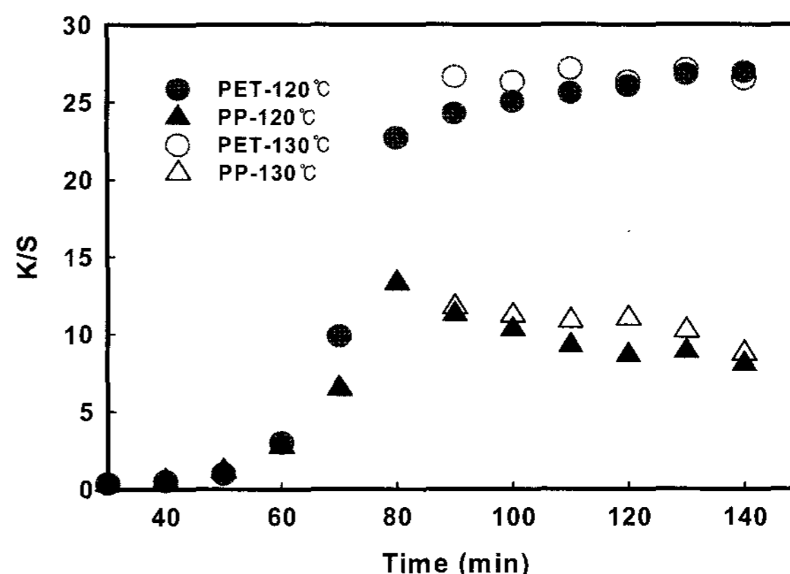
Fig. 1. K/S values of dyeable PP and PET dyed at 120°C and 130°C with dyeing time.
