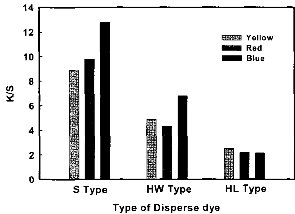
Fig. 4. K/S values of PET/dyeable PP double knit fabric dyed with three types of disperse dyes at 2%owf.
