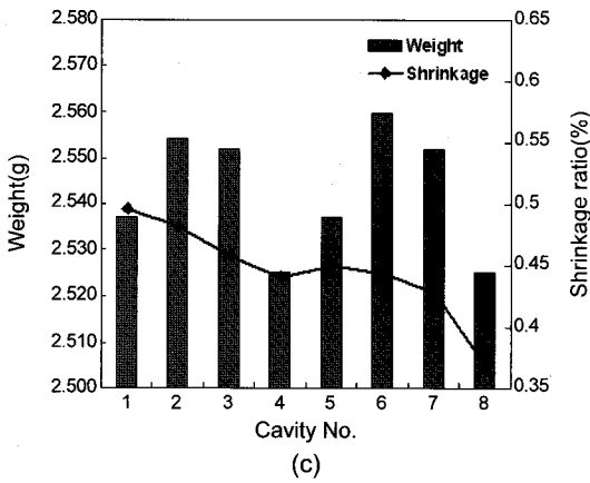
Figure 14. Variations of shrinkages and weights of parts for PC. (a) Speed 50 mm/sec, (b) speed 150 mm/sec, and (c) speed 250 mm/sec.
