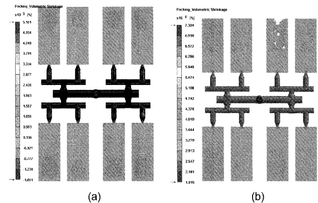
Figure 17. Computer simulation of shrinkage distribution. (a) PC at 150 mm/sec and (b) Zeonex at 150 mm/sec.
