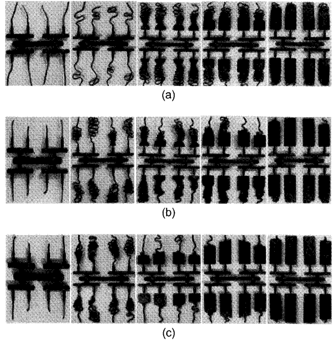
Figure 5. Flow patterns of PC according to injection speed. (a) Short shot experiment for speed of 50 mm/sec, (b) short shot experiment for speed of 150 mm/sec, and (c) short shot experiment for speed of 250 mm/sec.
