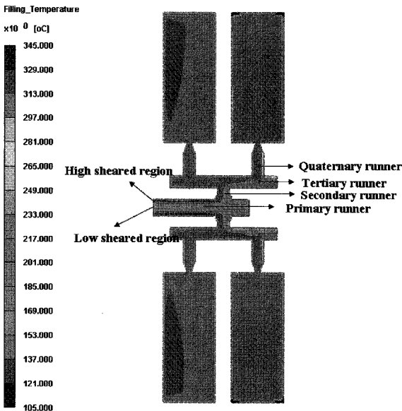
Figure 7. Computer simulation of temperature distribution in runner for PC at 150 mm/sec.
