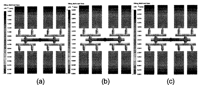
Figure 11. Computer simulation of flow pattern for various injection speeds for Zeonex. (a) Speed 10 mm/sec, (b) speed 50 mm/sec, and (c) speed 250 mm/sec.
