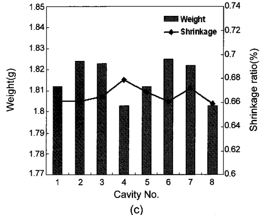
Figure 15. Variations of shrinkages and weights of parts for Zeonex. (a) Speed 10 mm/sec, (b) speed 50 mm/sec, and (c) speed 250 mm/sec.
