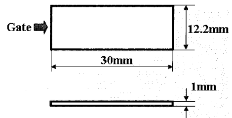
Figure 2. Dimension of cavity.
