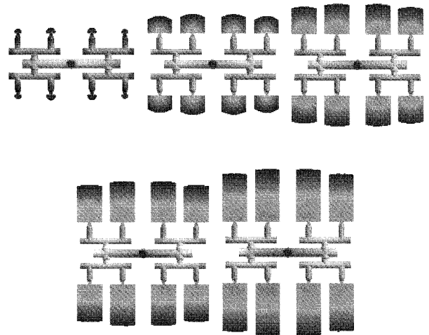
Figure 6. Computer simulation of flow pattern of PC for speed of 150 mm/sec.
