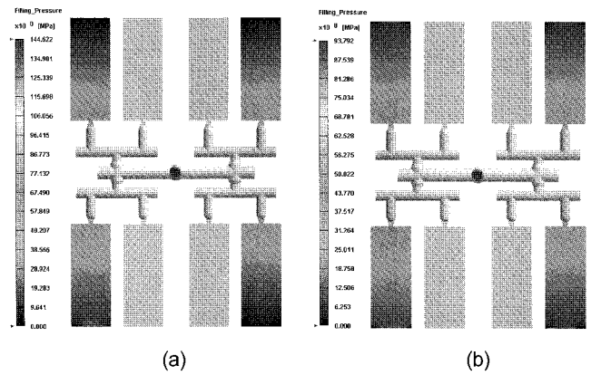
Figure 16. Computer simulation of pressure distribution. (a) PC at speed 150 mm/sec and (b) Zeonex at speed 250 mm/sec.
