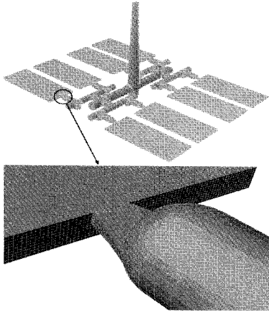
Figure 4. 3D mesh in runner and cavities for simulation.
