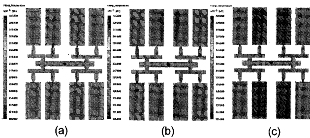
Figure 9. Computer simulation of temperature distribution for various injection speeds for PC. (a) Speed 50 mm/sec, (b) speed 150 mm/sec, and (c) speed 250 mm/sec.
