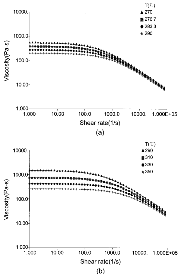
Figure 13. Viscosity curves of PC and Zeonex (Source: Moldflow). (a) PC Trirex 3025 GRU30 and (b) Zeonex E48R.
