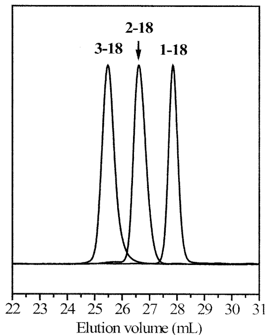
Figure 1. GPC curves of 1-18 , 2-18 and 3-18 .
