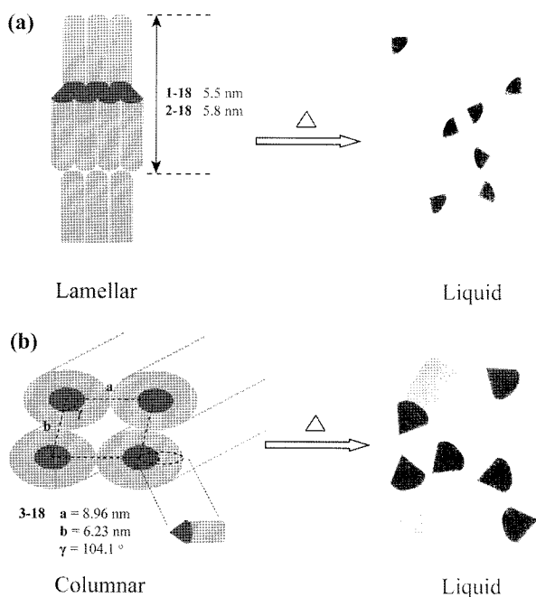
Figure 6. Schematic sketches of morphological transitions from (a) the lamellar structures of 1-18/2-18 and (b) oblique columnar structure of 3-18 to isotropic liquid states upon heating.
