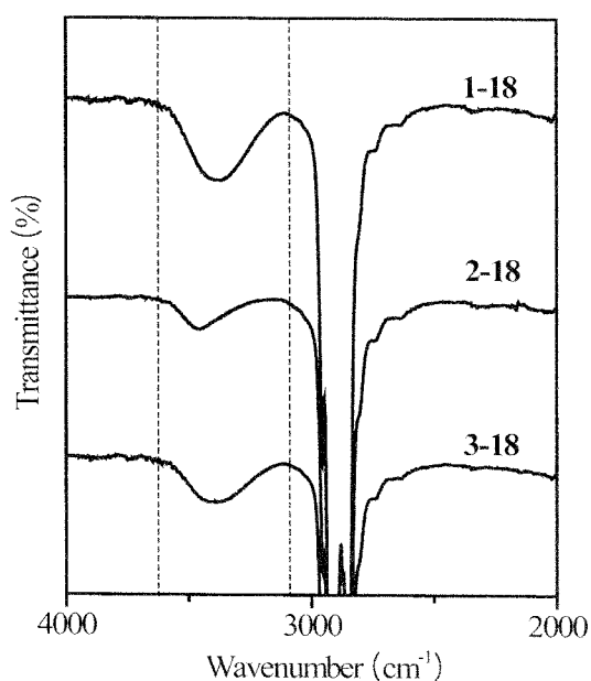
Figure 4. IR spectra of 1-18 , 2-18 , and 3-18 . The dotted region corresponds to the absorption of hydrogen-bonded O-H stretching vibration.
