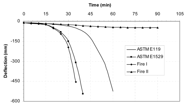
Fig. 15 Variation of deflection with fire exposure time for simply supported HSC beam (Permeability = 10^{-18} \text{ m}^2 ).
