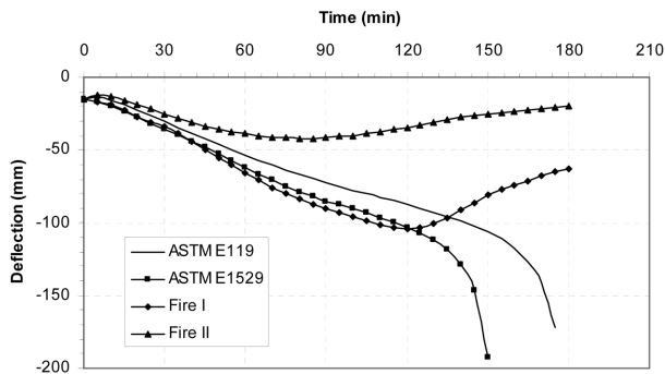
Fig. 14 Variation of deflection with fire exposure time for axially restraint NSC beam.
