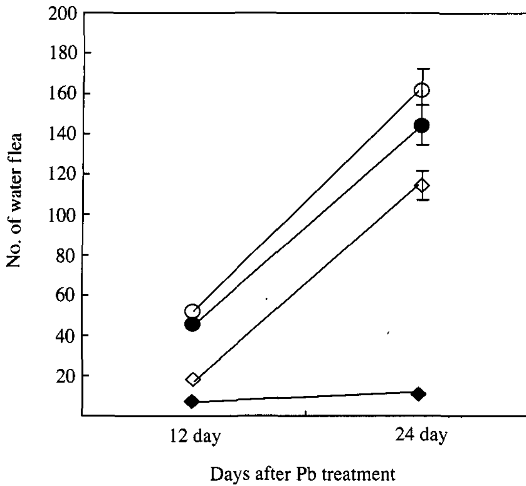
Fig. 3. Changes in individual numbers of water flea, Moina macrocopa , for reproduction impairment test with time courses under various concentrations of lead treatment to media (○: -0, ●: -10, ◇: -100, ◆: -200 µg/L) Bars indicate S.D.
