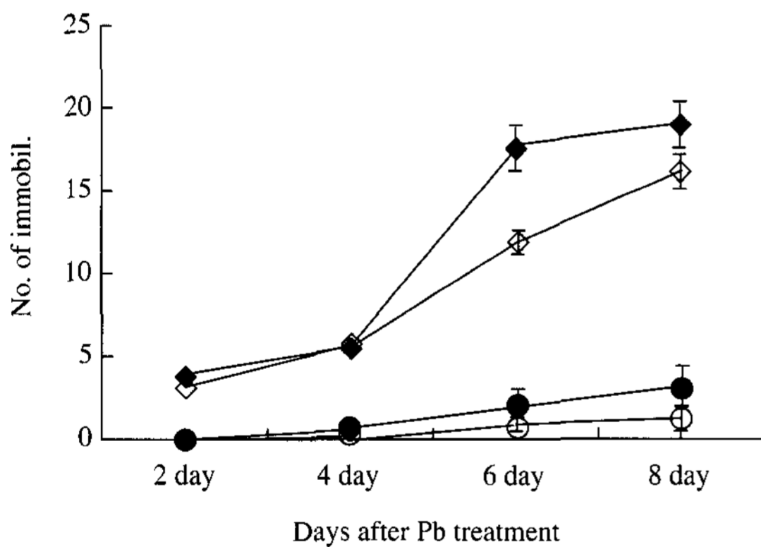
Fig. 1. Changes in immobilized numbers of water flea, Moina macrocopa , for immobilization test with time coursed under various concentrations of lead (Pb) treatment to media (○: -0, ●: -0.1, ◇: -1.0, ◆: -2.0 mg/L). Bars indicate S.D.
