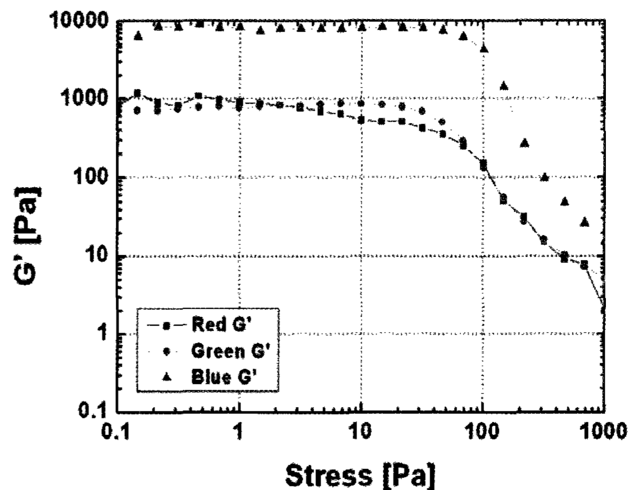
Figure 11. Shear stress dependent of G' for low viscosity type millbase (stress range : 0.1~1,000 Pa).
