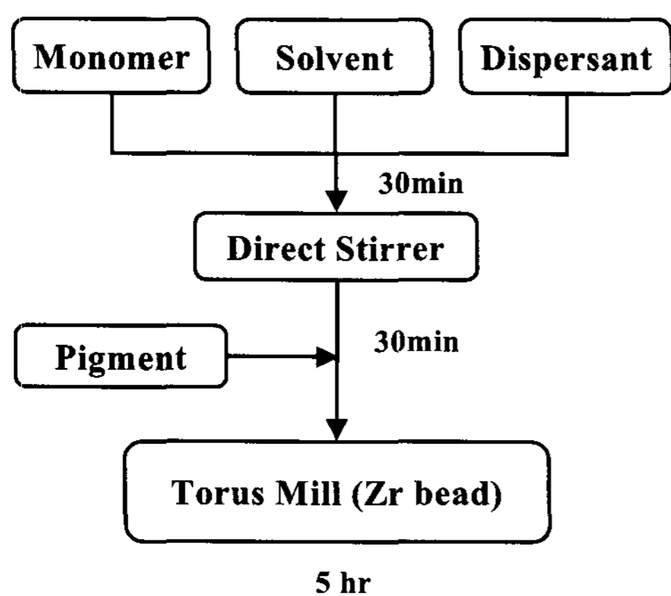
Figure 2. Schematic of millbase process.
