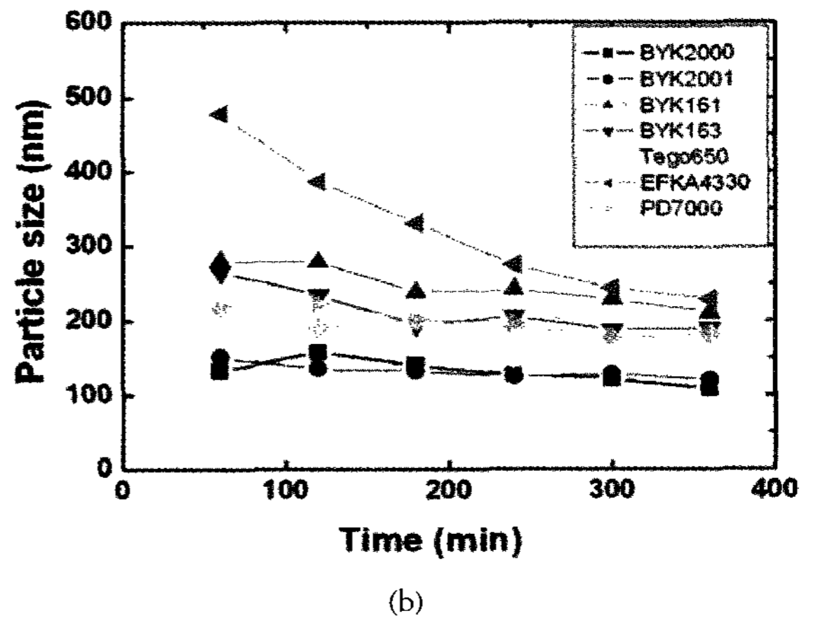
Figure 3. Particle size measured versus dispersant mixing time (C. I. Pigment Red 177 (a) C. I. Pigment Red 254 (b)).
