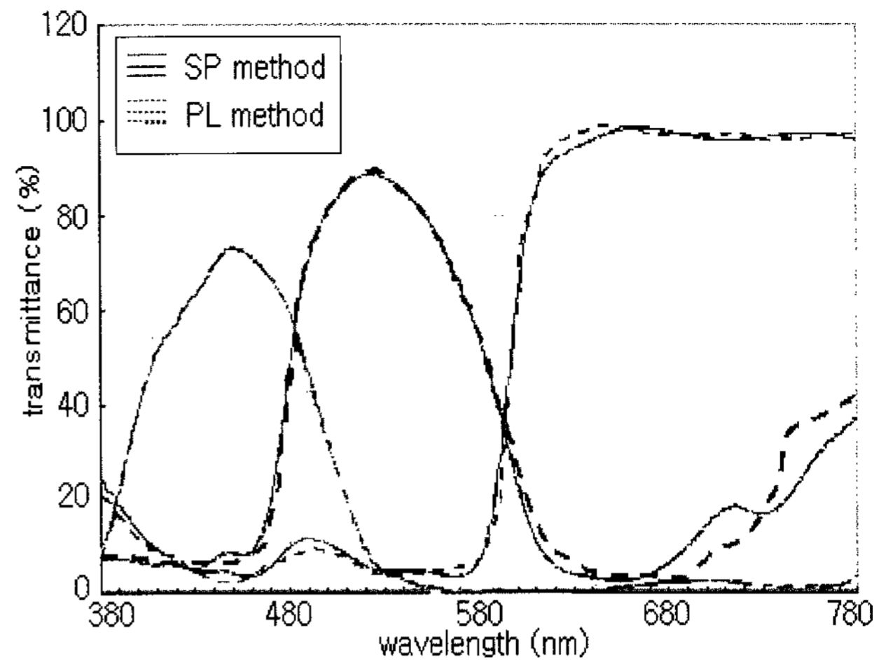
Figure 13. Transmittance ratio of R, G, B color resist at photolithography (PL) method. (Red : 95%, Green : 90%, Blue : 80%, thickness : 2.0 \mu\text{m} ) and Screen printing (SP) method. (Red : 95%, Green : 90%, Blue : 70%, thickness : R(3.5 \mu\text{m} ), G(2.5 \mu\text{m} ))
