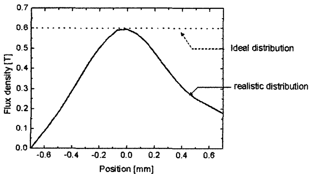
Fig. 6 Flux density along the airgap
