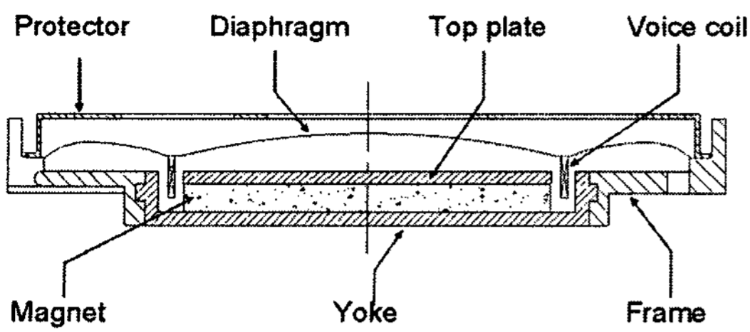
Fig. 1 Schematic of analyzed microspeaker
