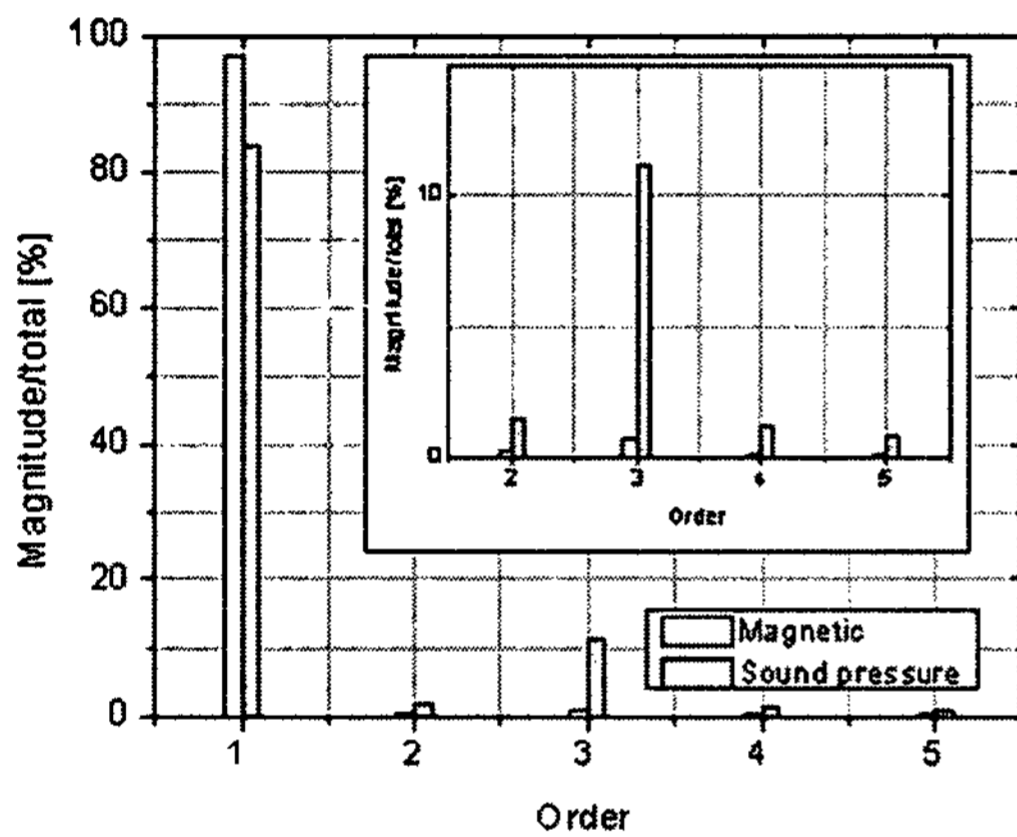
Fig. 18 Spectrum of force and pressure at 300 Hz
