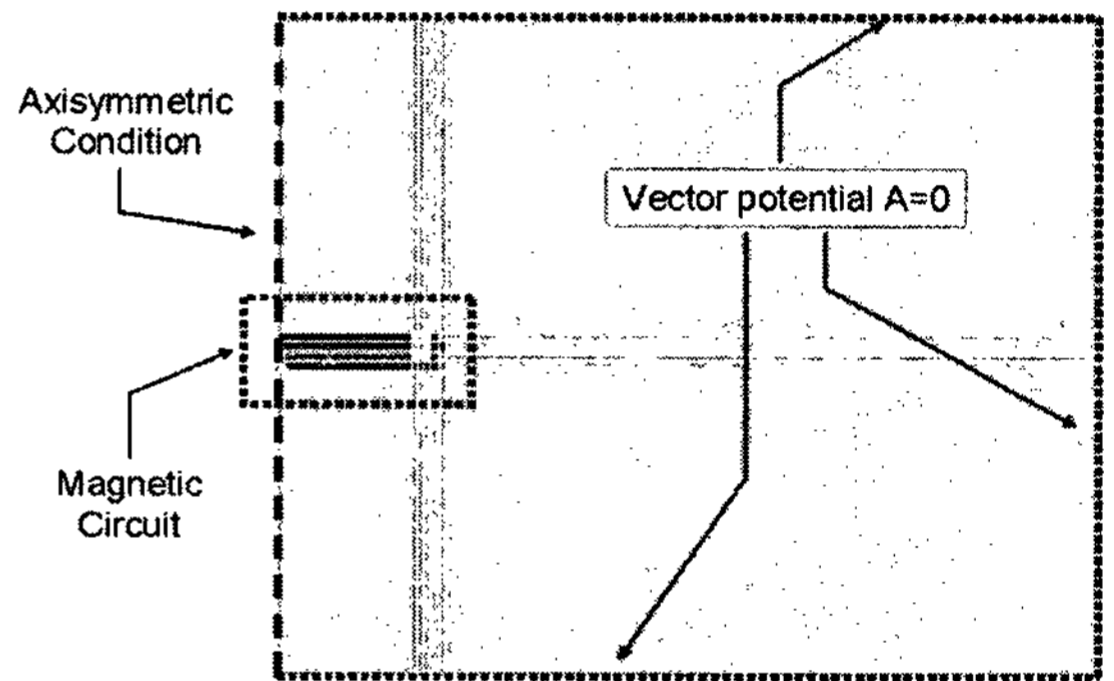
Fig. 3 Boundary condition of electromagnetic system
