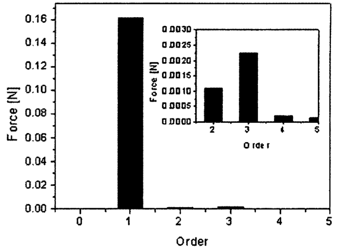
Fig. 15 Spectrum of magnetic force at 300 Hz
