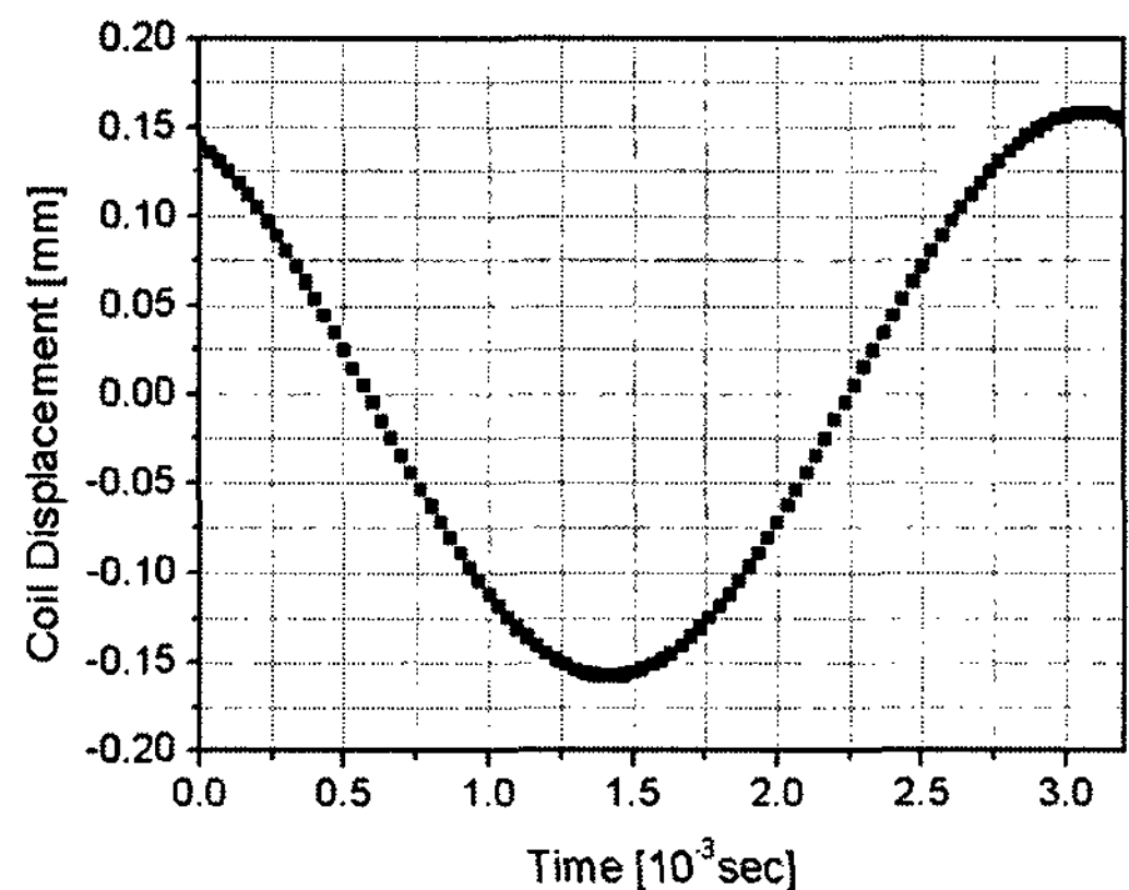
Fig. 12 Coil displacement when force is 0.1 N
