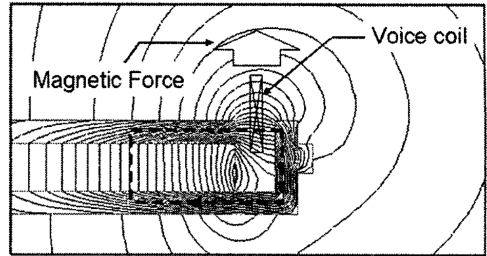
Fig. 2 Operating principle of microspeaker
