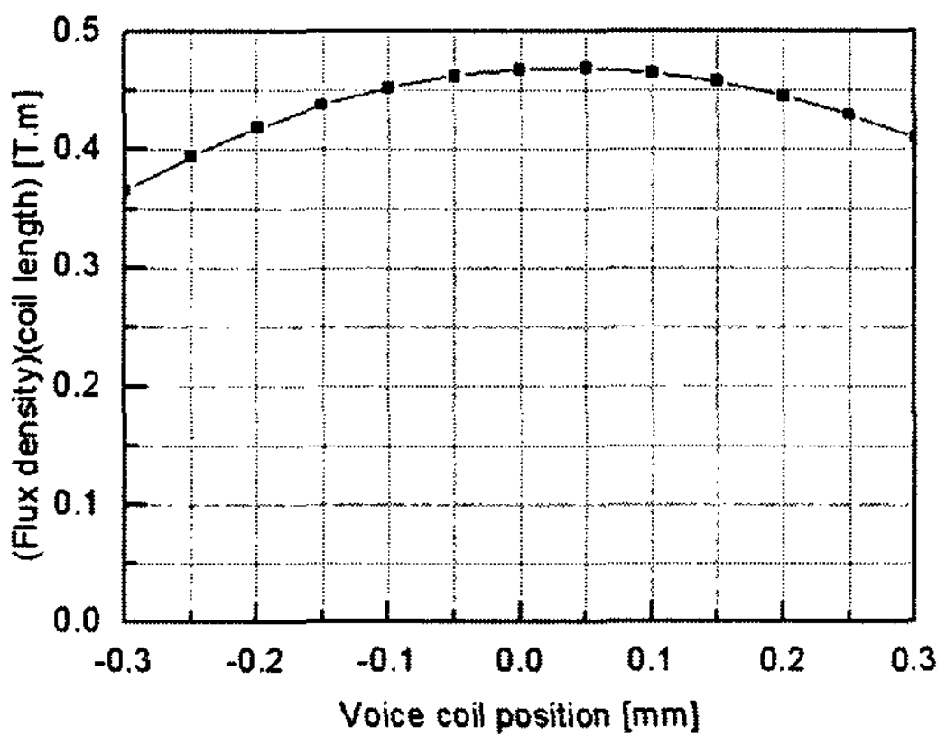
Fig. 10 Magnetic force per current
