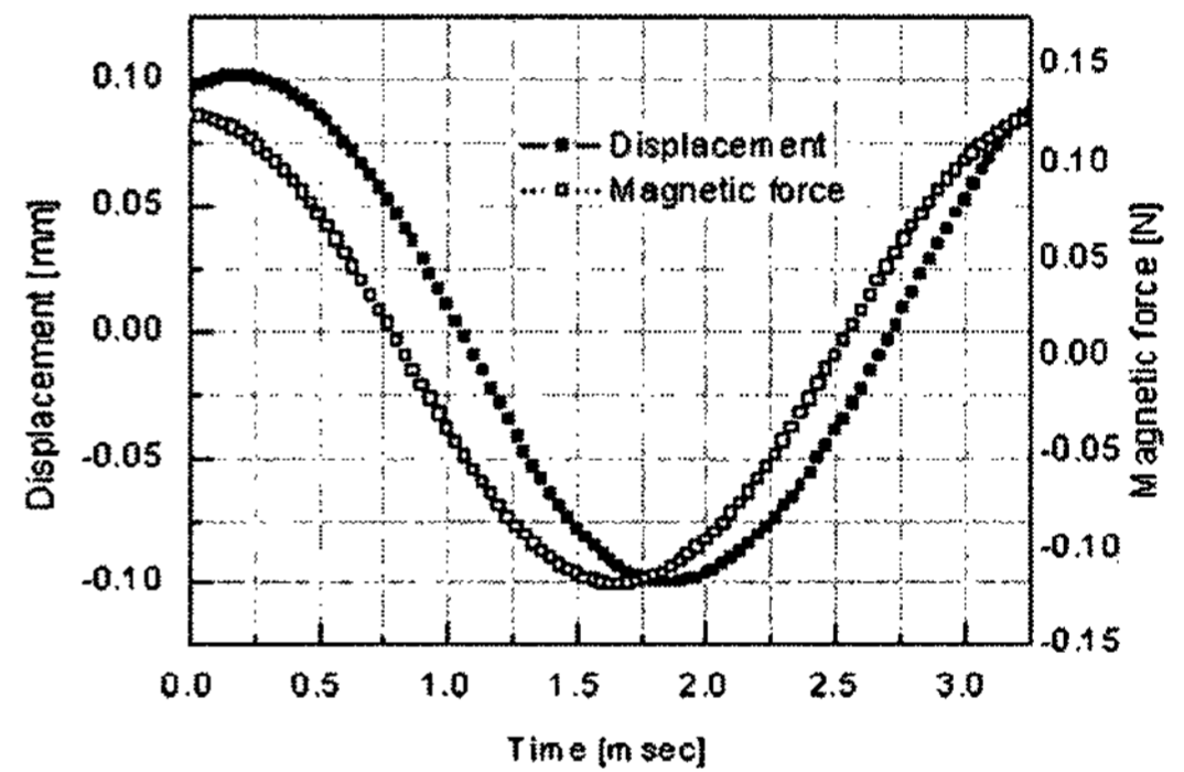
Fig. 16 Final solution of force and displacement at 300 Hz
