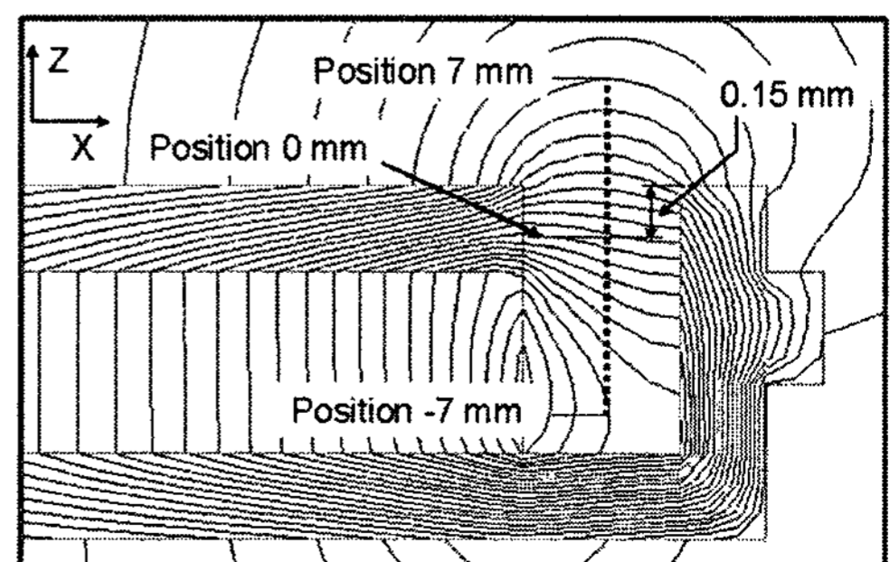
Fig. 5 Fluxlines and definition of position
