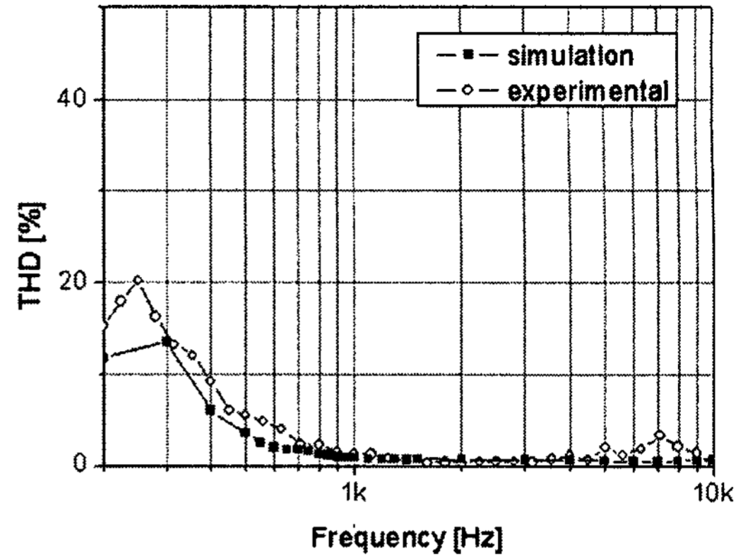
Fig. 19 Total harmonic distortion
