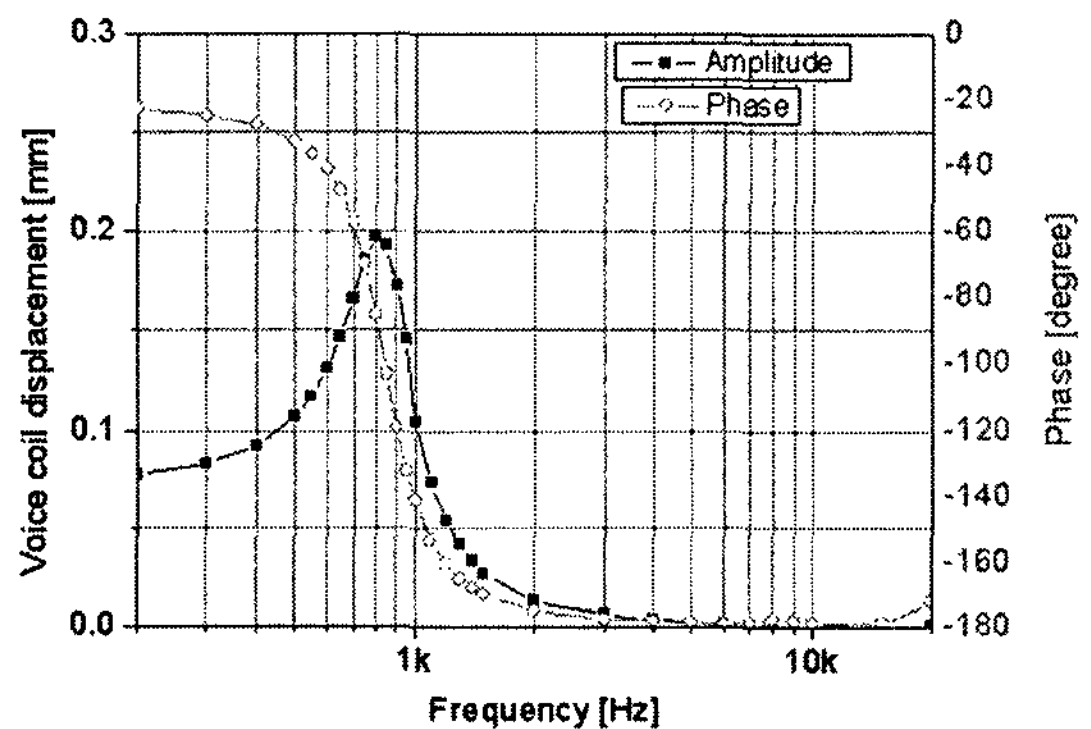
Fig. 8 Voice coil displacement
