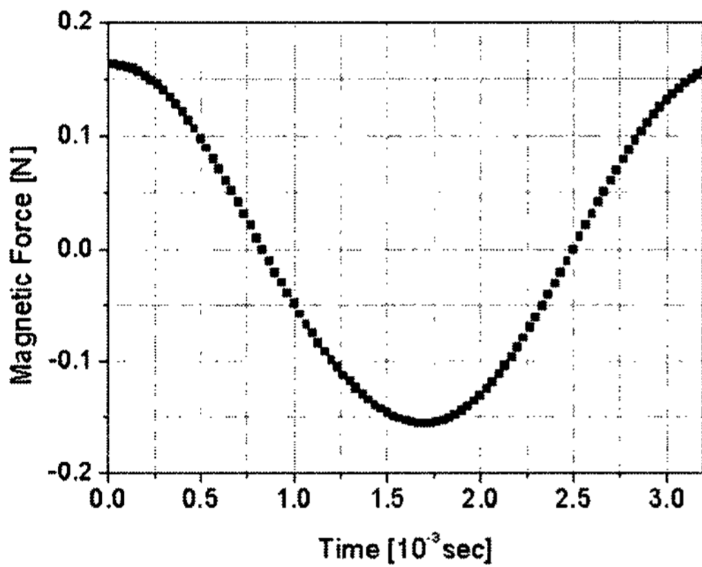
Fig. 14 Magnetic force at 300 Hz
