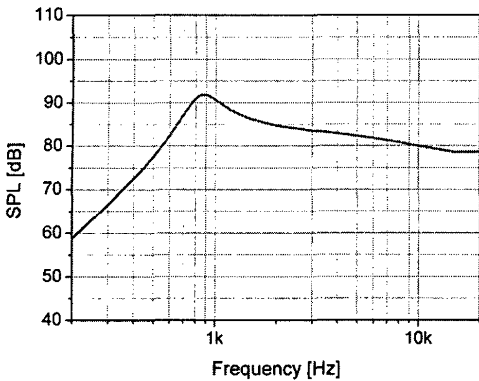
Fig. 9 Sound pressure level
