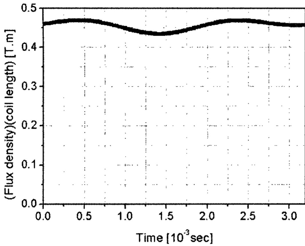
Fig. 13 Magnetic force per current at 300 Hz
