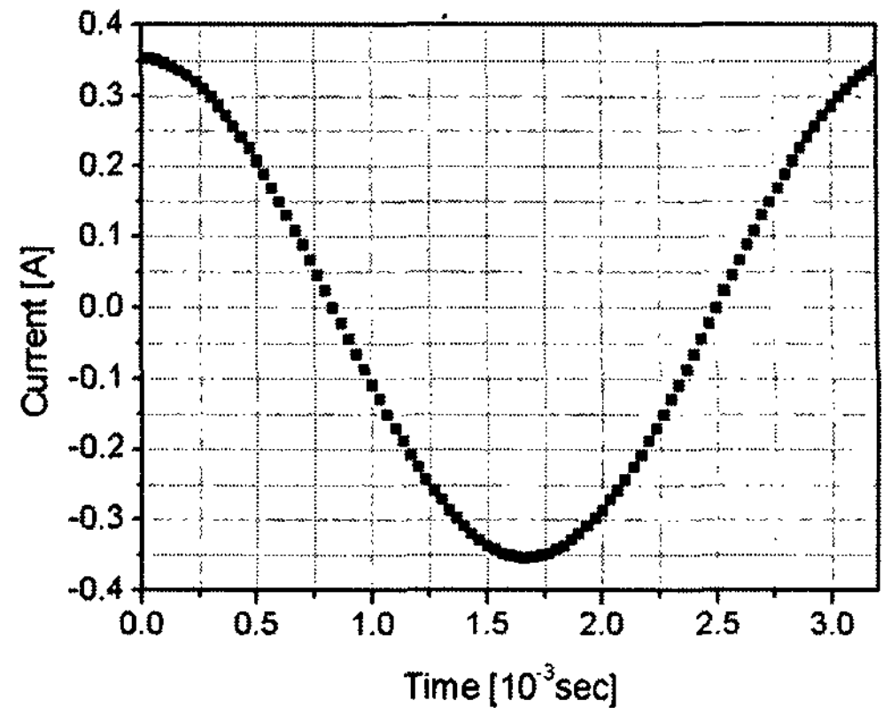
Fig. 11 Current on voice coil at 300 Hz
