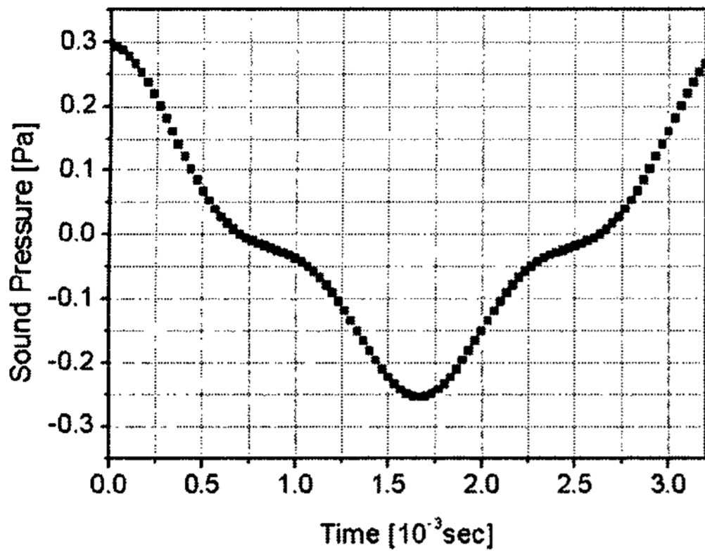
Fig. 17 Sound pressure at 300 Hz
