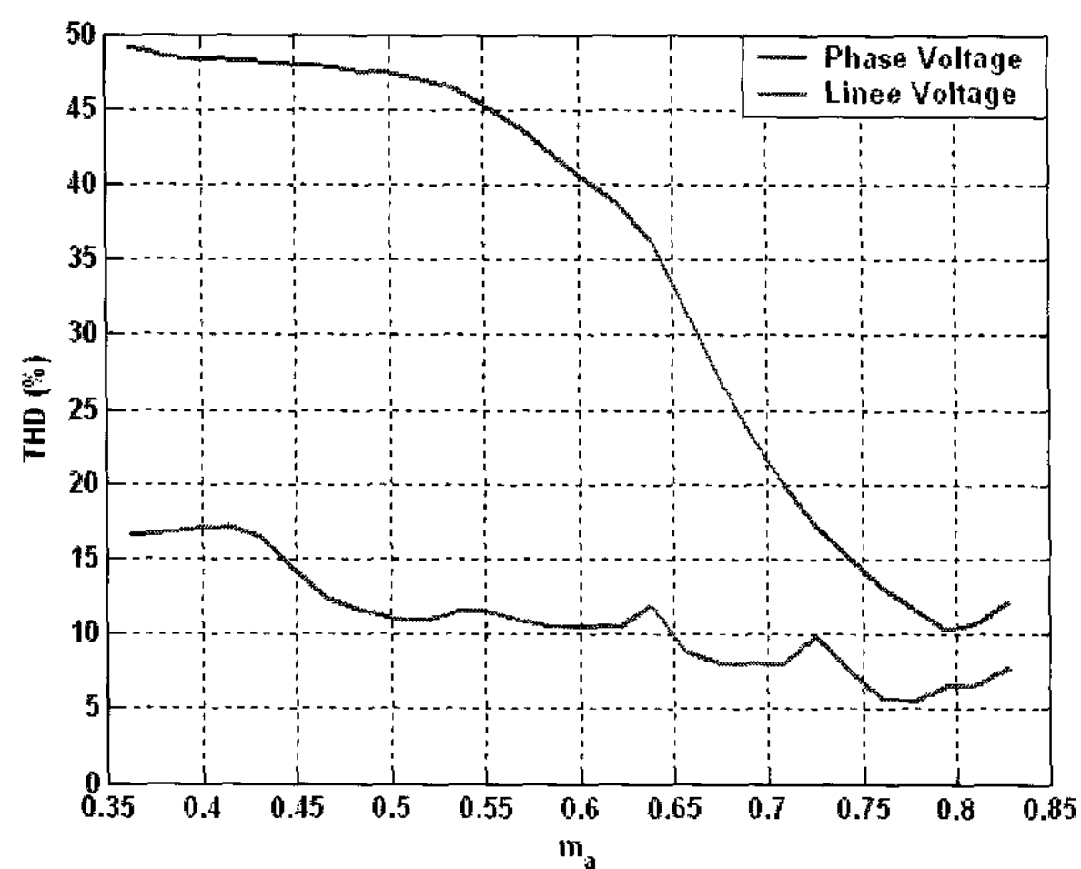
Fig. 6 Phase and line voltage THD as a function of m_a for seven-level inverter (OMTHD technique)
