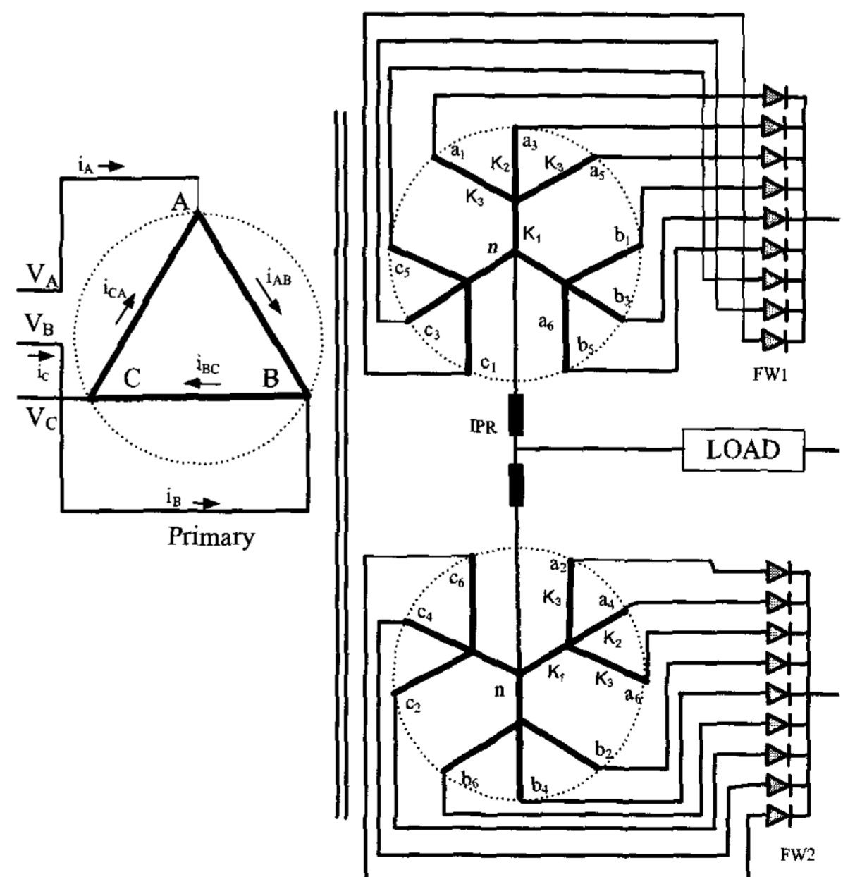
Fig. 4a Delta/ double fork transformer winding arrangement for 18-phase full-wave AC-DC conversion
