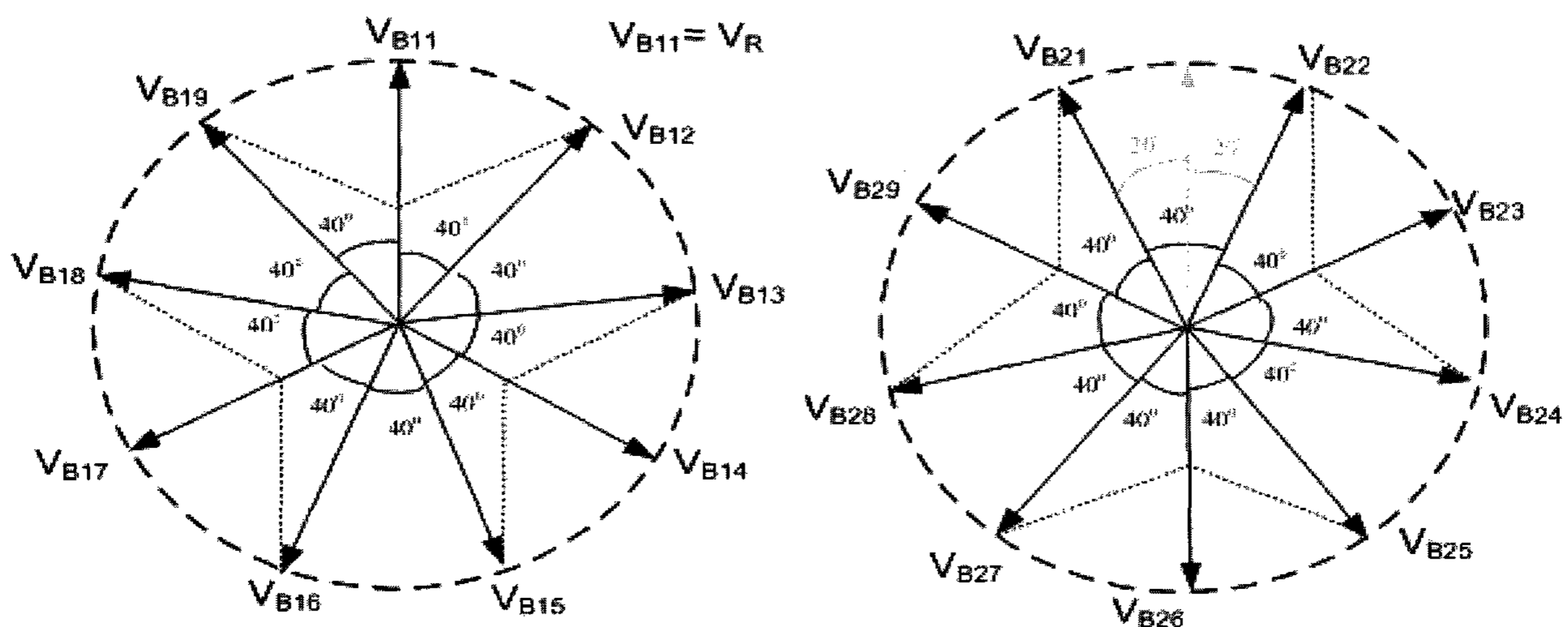
Fig. 4b Graphical representation of delta/double fork transformer secondary windings for 18-pulse AC-DC converter and phasor diagram
