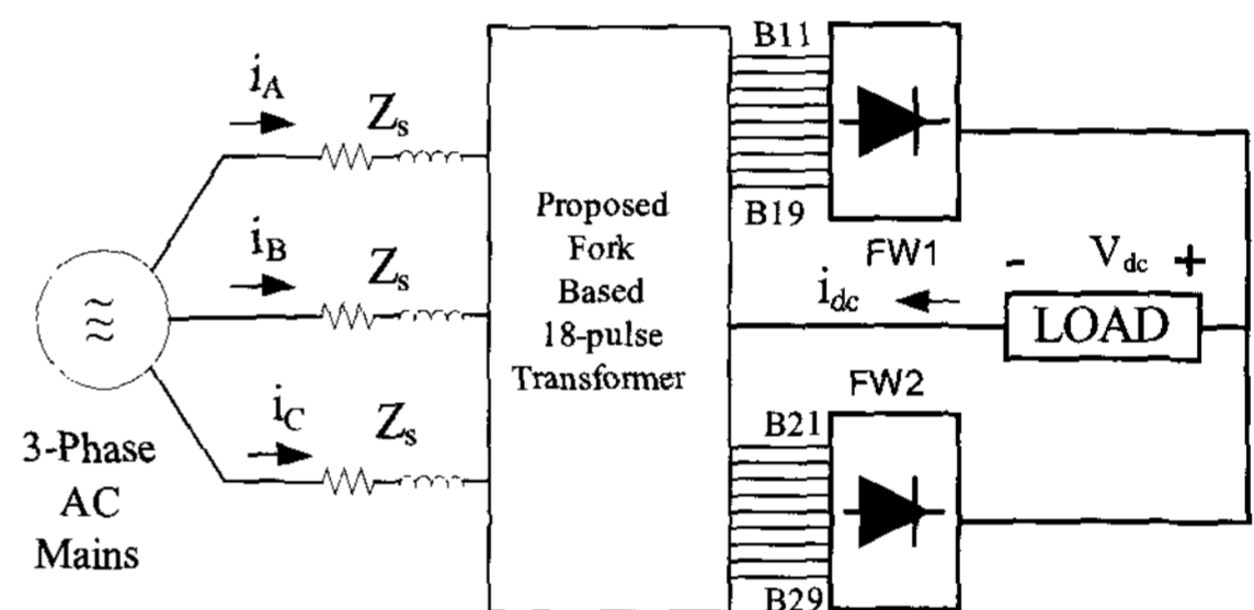
Fig. 3 Proposed delta/fork transformer based 18-pulse AC-DC converter
