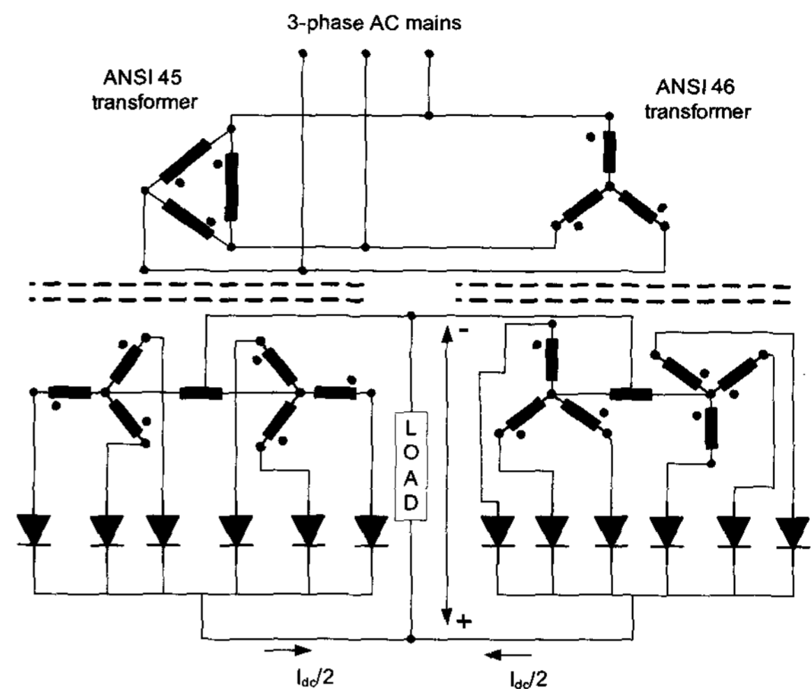
Fig. 2 A delta/double star transformer (ANSI 45) and star/double star transformer (ANSI 46) combination for 12-pulse full-wave AC-DC conversion
