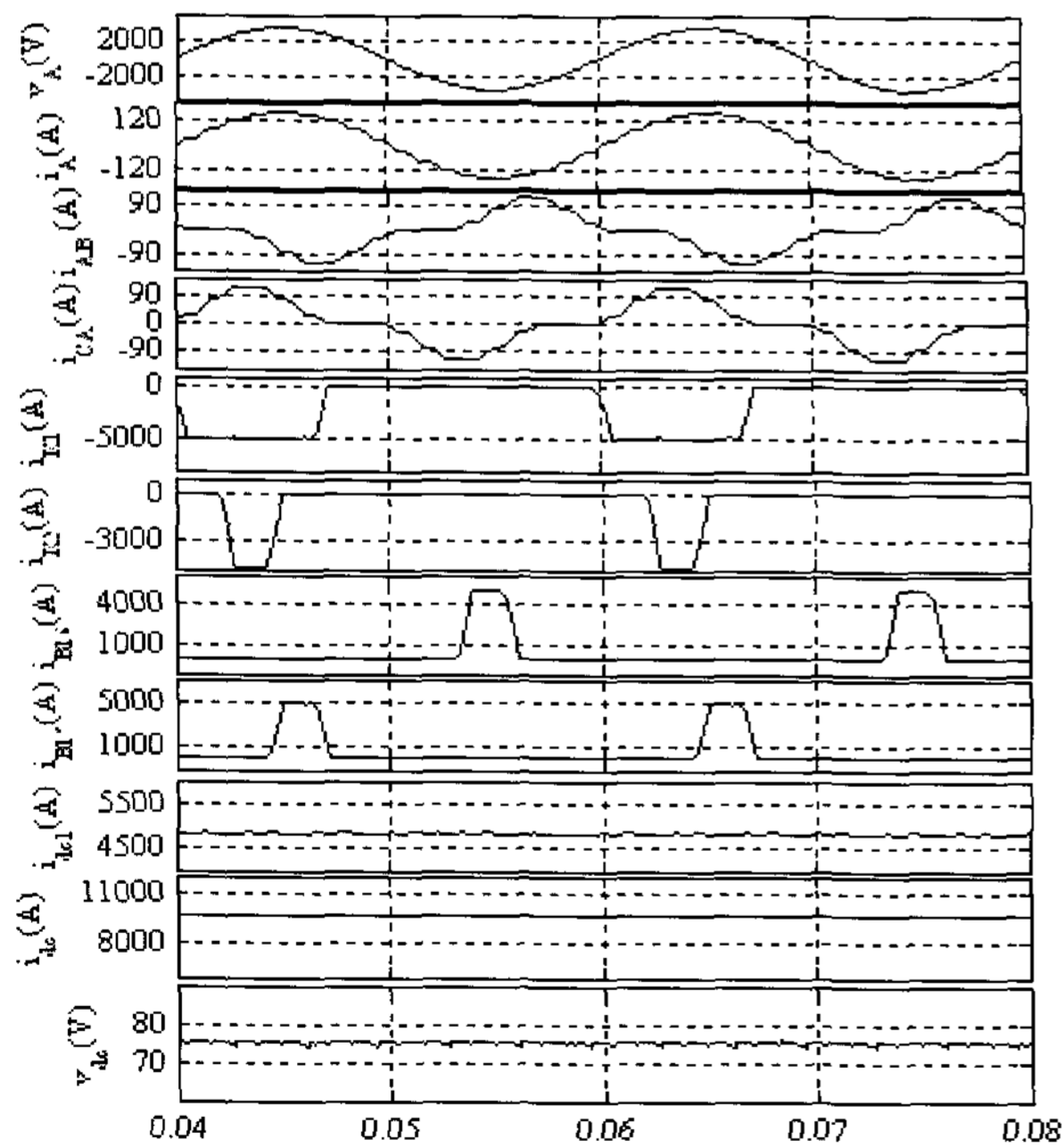
Fig. 7 Instantaneous values of input phase voltage ( V_A ), input AC mains current ( i_A ), primary winding currents ( i_{AB} and i_{CA} ), winding-currents of secondary ( i_{K1} , i_{K2} , i_{B15} , i_{B16} ), a bridge output current ( i_{dc1} ) and output DC current ( i_{dc} ) and voltage ( V_{dc} ) waveform of 18-pulse full-wave AC-DC converter at light-load
