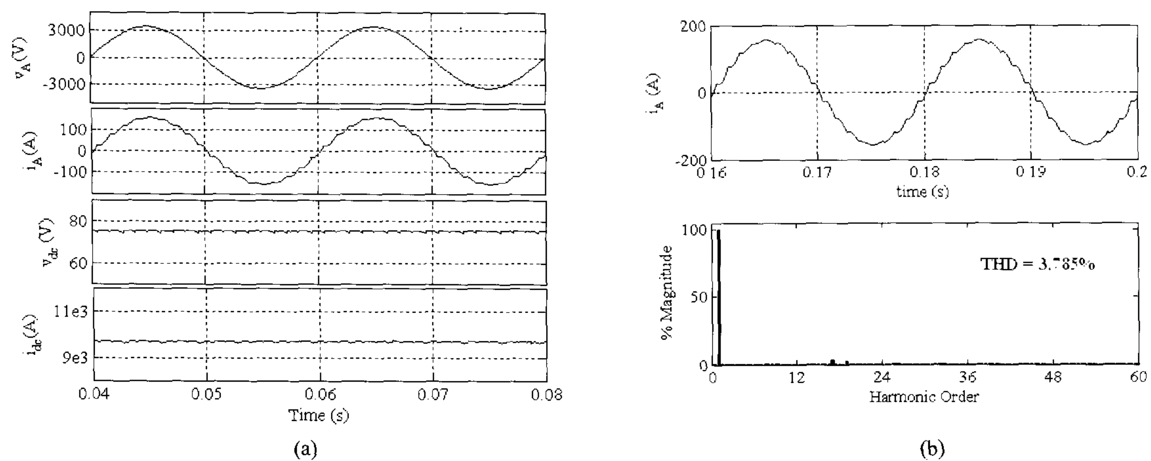
Fig. 12 Eighteen-pulse full-wave AC-DC converter at light-load - (a) Input and output voltage and current waveform (b) Input current waveform and its harmonic spectrum
