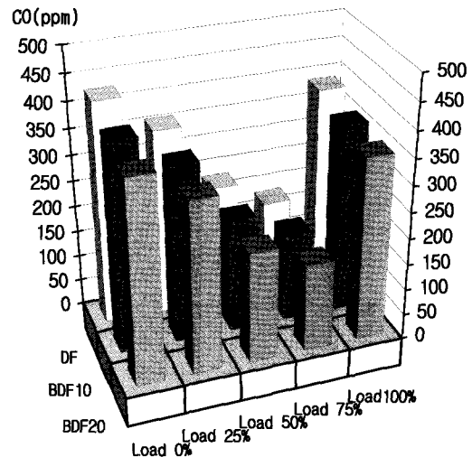
Fig. 3. CO emission characteristics at various engine loads.
