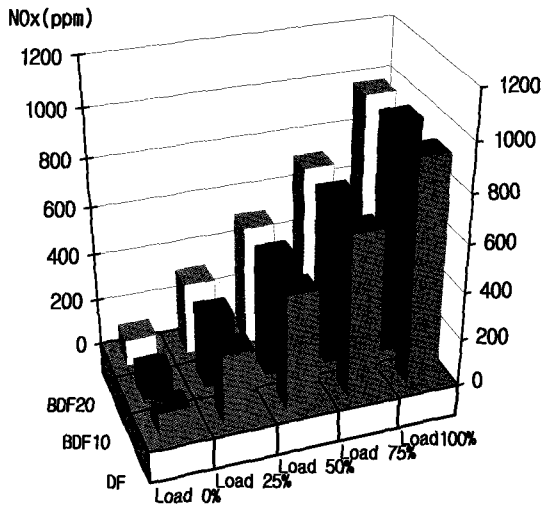
Fig. 4. NO x emission characteristics at various engine loads.
