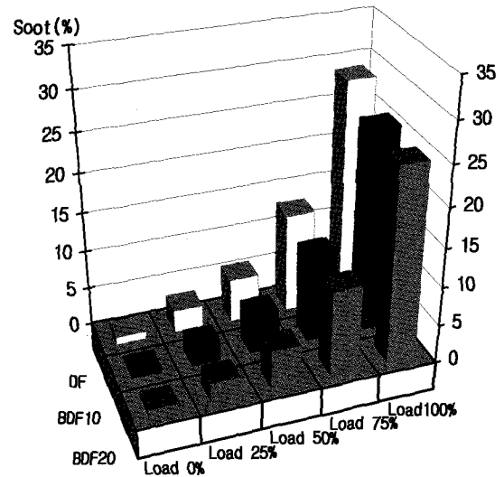
Fig. 5. Soot emission characteristics at various engine loads.
