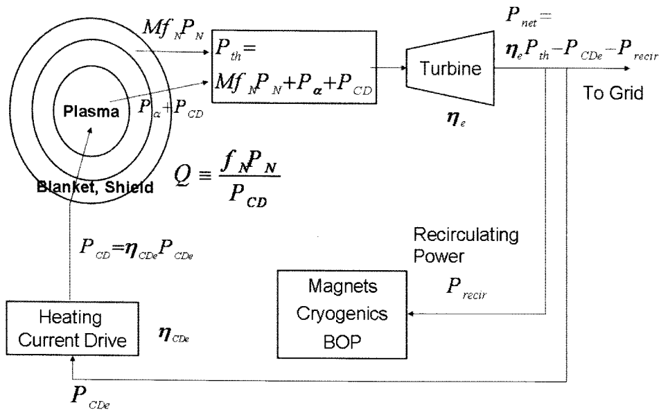
Fig. 2. Power Flow in a Tokamak Fusion Power Plant
