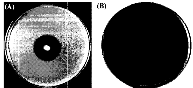
Fig. 4. Hydrolysis of protein (A) and starch (B) by strain KM1-15.
