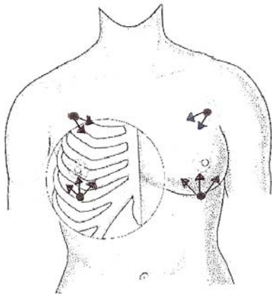
Fig. 1. Needle-embedding point(Jahyungchim)
