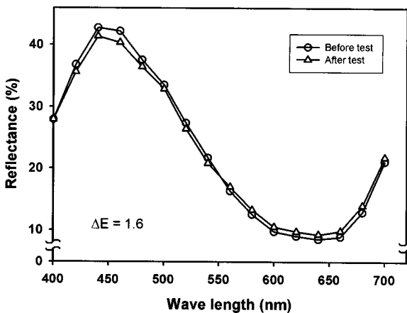
Fig. 5. Reflectance of 100% polyester fabric before and after light fastness test.
