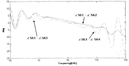
(b) Port 6 결과 (b) Results at Port 6
