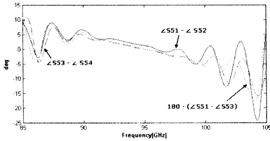
(a) Port 5 결과 (a) Results at Port 5
