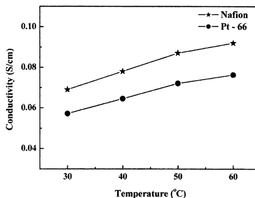
Fig. 4. Effect of the operating temperature on the ionic conductivity.
