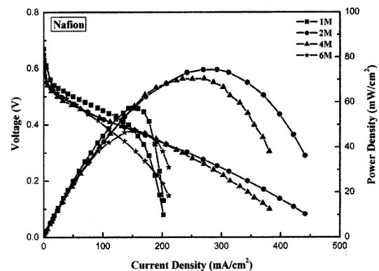
Fig. 7. Effect of the Pt-layer on the cell performance according to the methanol concentration ( \text{O}_2 , 30°C).
