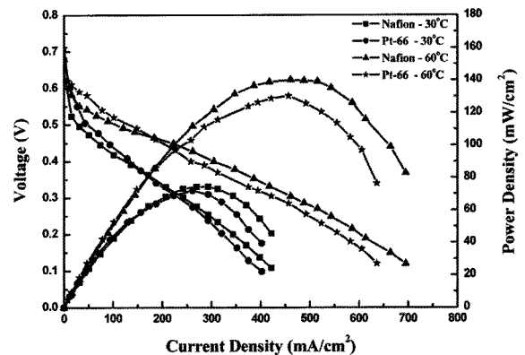
Fig. 6. Effect of the Pt-layer on the cell performance according to the operating temperature (2 M-methanol, \text{O}_2 ).
