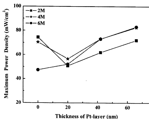
Fig. 8. Plot of maximum power density versus Pt-layer thickness on Nafion membrane as a function of methanol concentration.
