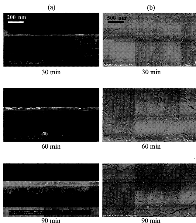
Fig. 1. SEM images of Pt-layers with different sputtering time: (a) cross-section of the Pt-layer deposited on silicon plate, and (b) surface of the Pt-layer on Nafion membrane.
