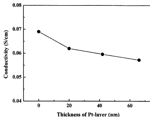
Fig. 3. Effect of the Pt-layer thickness on the proton conductivity in the modified membrane (30°C).
