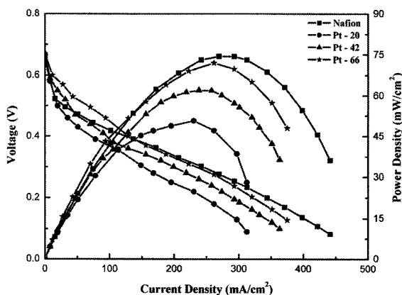
Fig. 5. Effect of the Pt-layer thickness on the cell performance (2 M-methanol, \text{O}_2 , 30°C).
