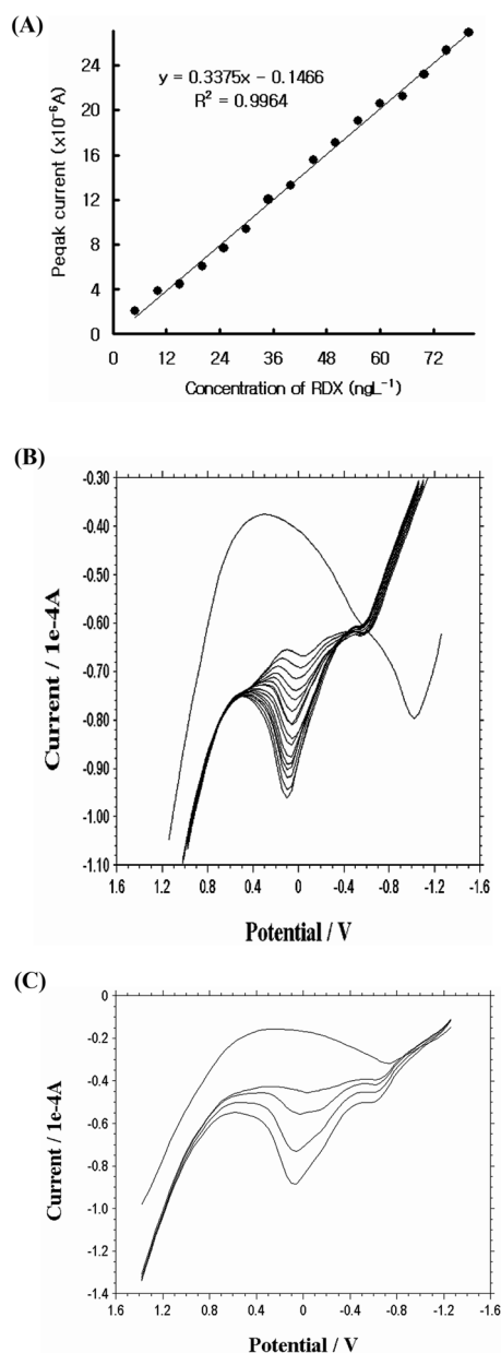
Fig. 3. (A): analytical linear ranges; and (B): raw voltammograms of 5, 10, 15, 20, 25, 30, 35, 40, 45, 50, 55, 60, 65, 70, 75, and 80 ng/L RDX in a 0.1 M \text{NH}_4\text{H}_2\text{PO}_4 electrolyte solution; (C): analytical application of the contaminated soil sample, each curve shown for the electrolyte blank solution, 0.05 mL soil solution spike, and standard for 10, 20, 30 ng/L RDX spike in a pH 6.1, in a 0.1 M \text{NH}_4\text{H}_2\text{PO}_4 , initial potential of -1.3 V, final potential of 1.4 V, SW frequency of 700 Hz, SW amplitude of 0.5 V, increment potential of 40 mV, and accumulation time of 300 s. Other parameters were used in Fig. 2.
