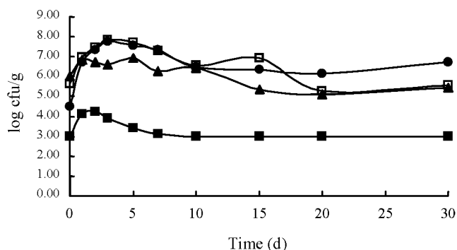
Figure 1. LAB (●), yeasts (□), bacillus (▲) and enterobacteria (■) counts of solid-state fermented feed during fermentation. Detectable level for enterobacteria (3.0 log cfu/g) was applied at day 10 and later days when no colony was detected on the plates.
