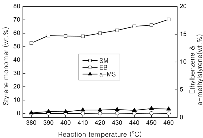
Fig. 7. Effect of reaction temperature on formation of styrene monomer, ethyl benzene and \alpha -methyl styrene.
