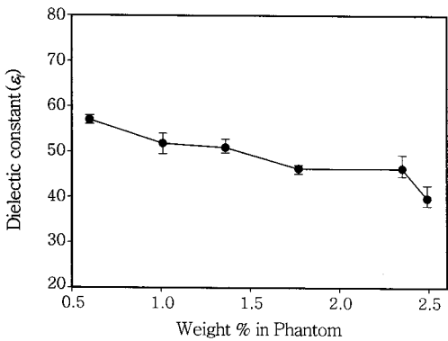
Figure 3. Dielectric constant of jelly phantoms as a function of sodium chloride content in phantom.
