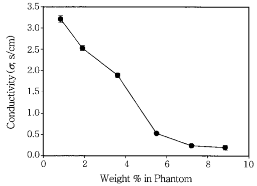
Figure 4. Conductivity of jelly phantoms as a function of polyethylene content in phantom.
