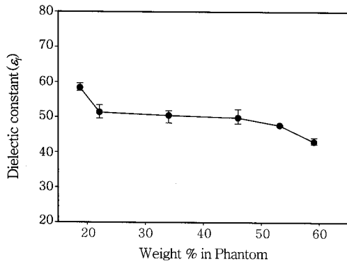
Figure 2. Dielectric constant of jelly phantoms as a function of deionized water content in phantom.
