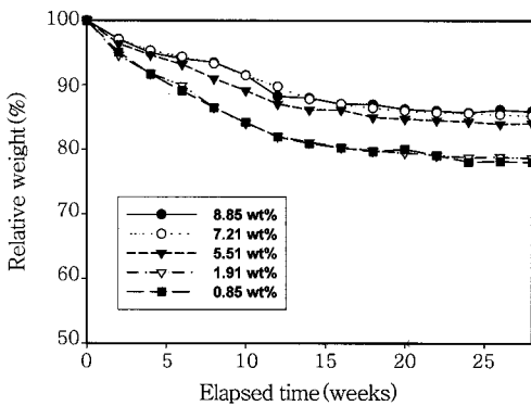
Figure 7. Change in the bulk weight of jelly phantoms containing various contents of polyethylene as a function of an elapsed time.
