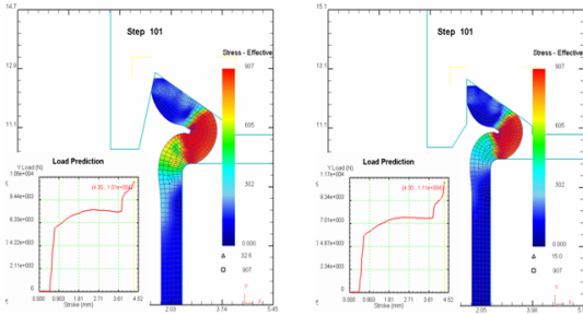
Fig. 5 Simulated load-stroke curve & Distribution of effective stress
