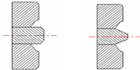
Fig. 3 Punching shape of cold forging dies
