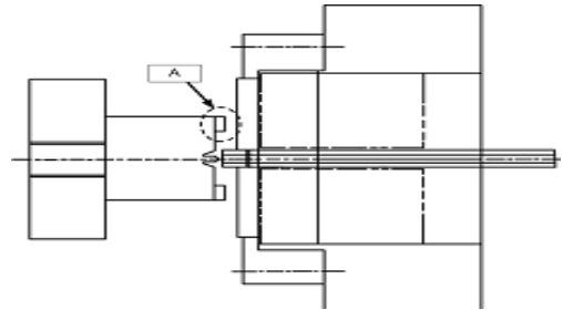
Fig. 2 Schematic drawing of the press used to form the pipe
