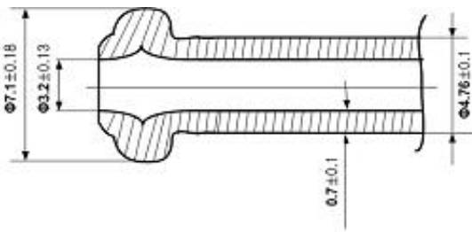
Fig. 1 Clamping part for brake pipe of automobiles drawing
