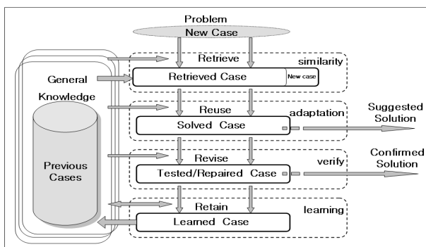
(그림 1) Case-based reasoning architecture
