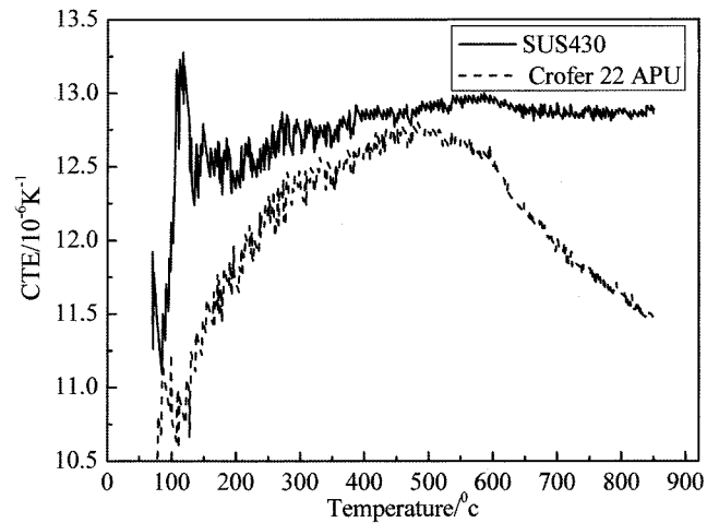
Fig. 2. Coefficients of thermal expansion of Crofer 22 APU and SUS430.
