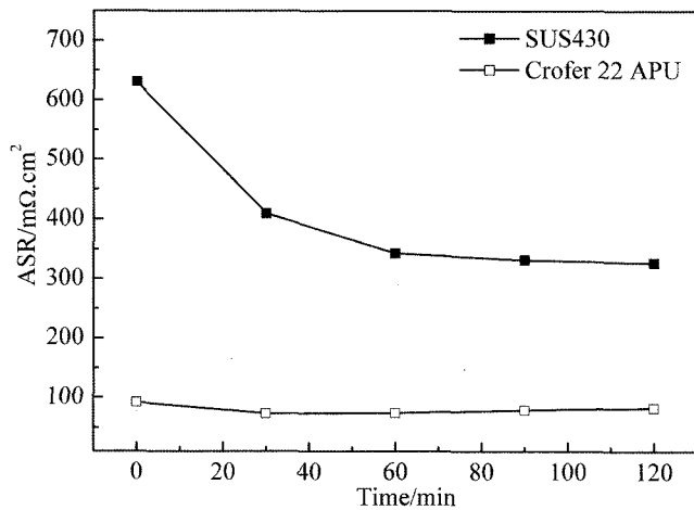
Fig. 9. Area-specific resistances of SUS 430 and APU LSM-coated by slurry spray as a function of holding time at 850°C.
