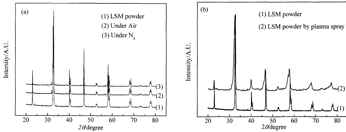
Fig. 8. XRD patterns of LSM powder and the LSM coating (a) by slurry spray; (b) by plasma spray.
