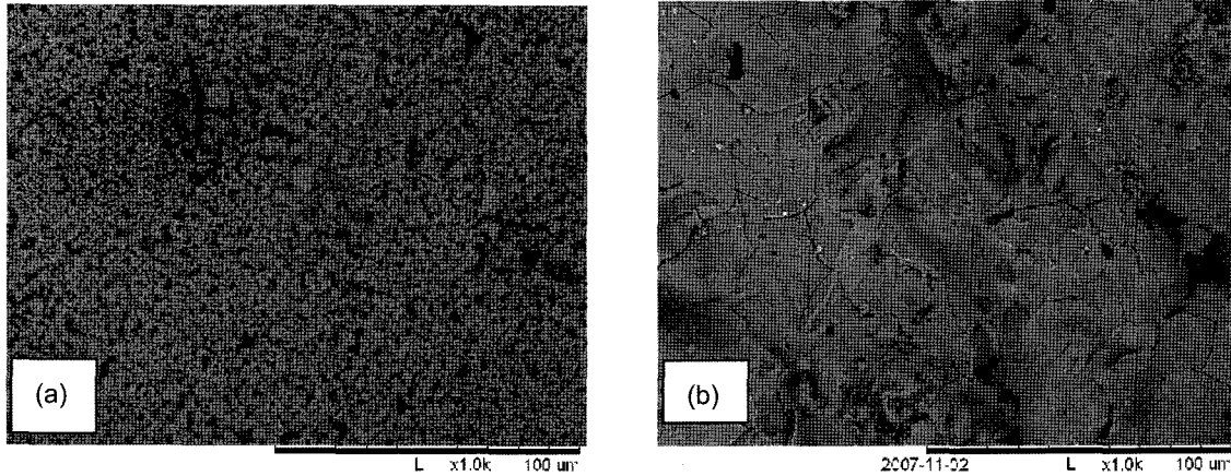
Fig. 7. SEM photographs of the surfaces of SUS430 and Crofer 22 APU with LSM coating (a) by slurry spray; (b) by plasma spray.
