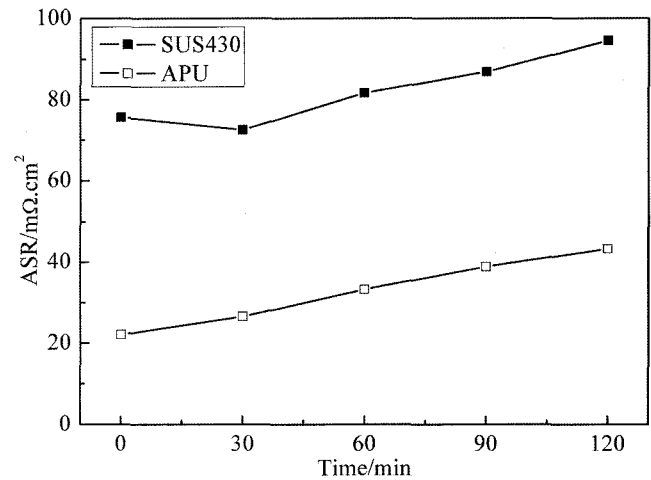
Fig. 10. Area-specific resistances of SUS 430 and APU LSM-coated by plasma spray as a function of holding time at 850°C.
