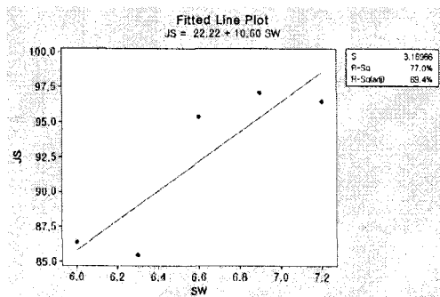
Fig. 11 Result of correlation and regression SW vs JS
