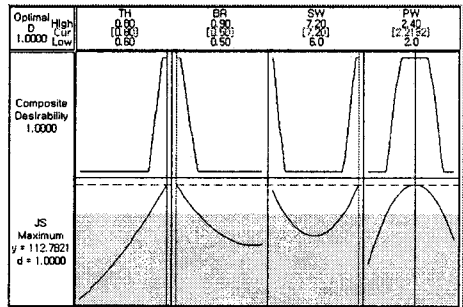
Fig. 15 Result of response surface optimize
