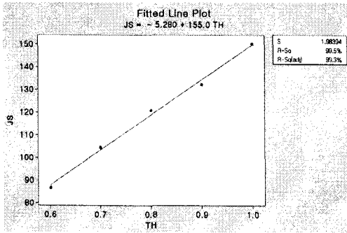
Fig. 9 Result of correlation and regression TH vs JS
