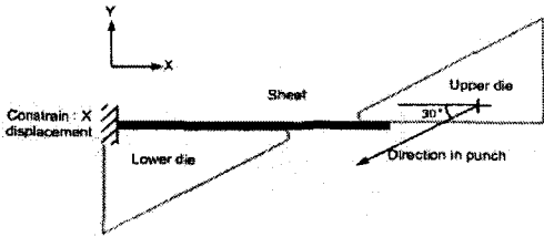
Fig. 6 F.E model and boundary condition of bending
