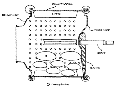
Fig. 3 Configuration of mechanical joining division
