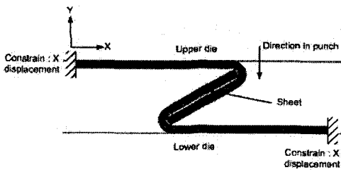
Fig. 7 F.E model and boundary condition of pressing
