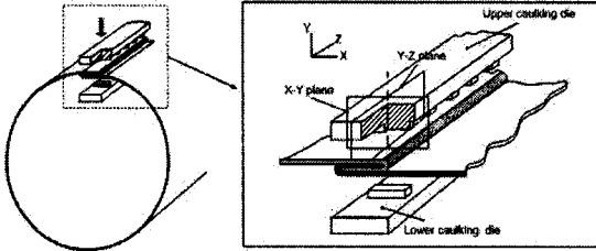
Fig. 4 Mechanical press-joining of spin drum
