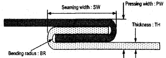
Fig. 5 Design factor and nomenclature
