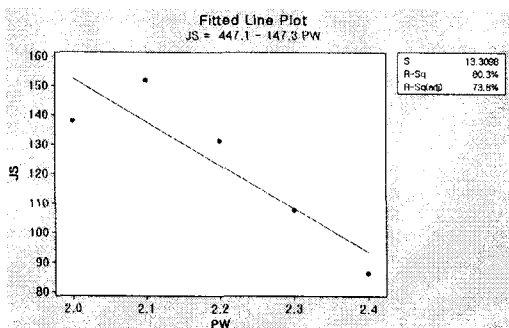
Fig. 12 Result of correlation and regression PW vs JS
