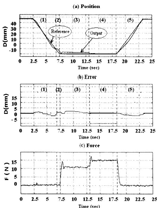
Fig. 7 Experimental Results about Grasping Test of Three-Finger Hand System
