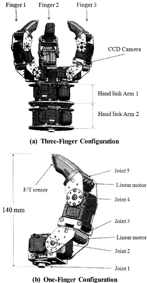
Fig. 3 The Structure of Three-Finger Hand System
