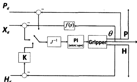
Fig. 4 The Scheme of the Position and Force Control
