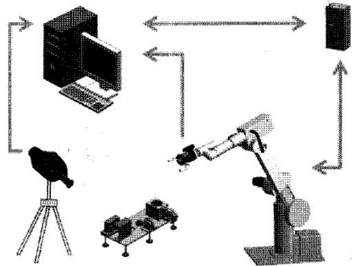
Fig. 2 The Overall Control System
