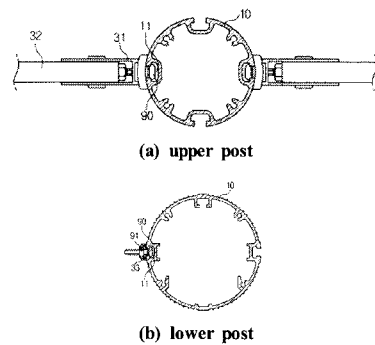
Fig. 2 Section of Aluminum Lighting Pole.
