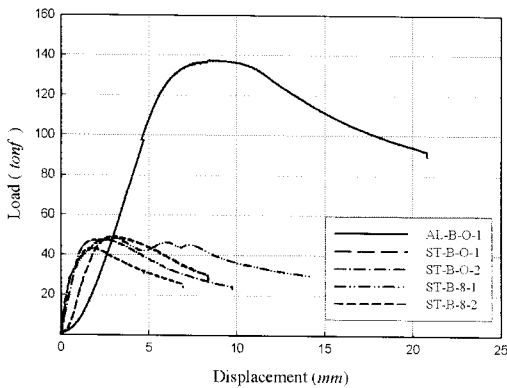
Fig. 5 Load-displacement curve.
