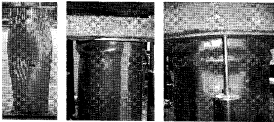
(a) AL-B-0 (b) ST-B-0 (c) ST-B-8
