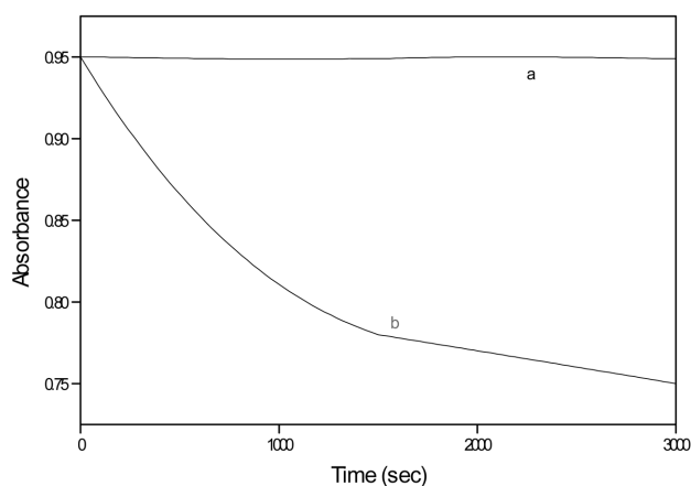
Fig. 4. Rhodamine B degradation followed by decrease of the absorbance at 552 nm at pH 8.1 in 10 mM phosphate buffer: (a) in presence of 0.1 mM [CuL^I](OAc)_2 ; (b) in presence of 0.1 mM [CuL^I](OAc)_2 , 1 mM H_2O_2 , 10 mM ascorbic acid.
