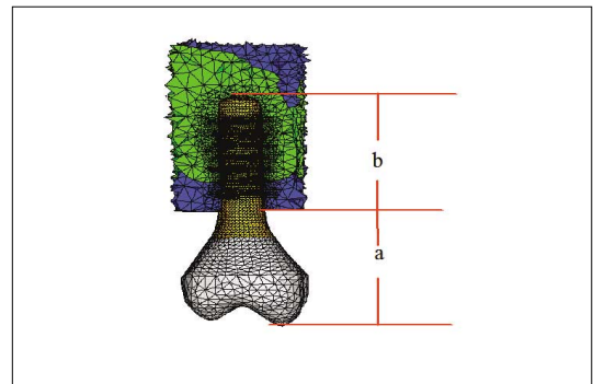
Fig. 2. Implant model to Crown/Fixture ratio: Model I 1 is 0.7:1; Model I 2 is 1:1; Model I 3 is 1.25:1.
