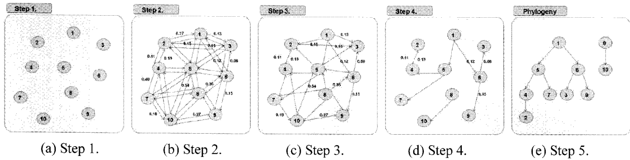
Fig. 2. Step 1 shows the 10 given programs. Step 2 involves computing the bi-directional evolutionary distances between node a and b , which is represented by double edges. Step 3 involves selecting a more plausible evolutionary edge. Step 4 involves constructing a minimal spanning tree in the under-graph of the directed graph given in (c). Step 5 involves applying our Spanning Forest Construction Algorithm to the minimal spanning tree obtained in (d). In Step 5, this forest is the final output of this work.
