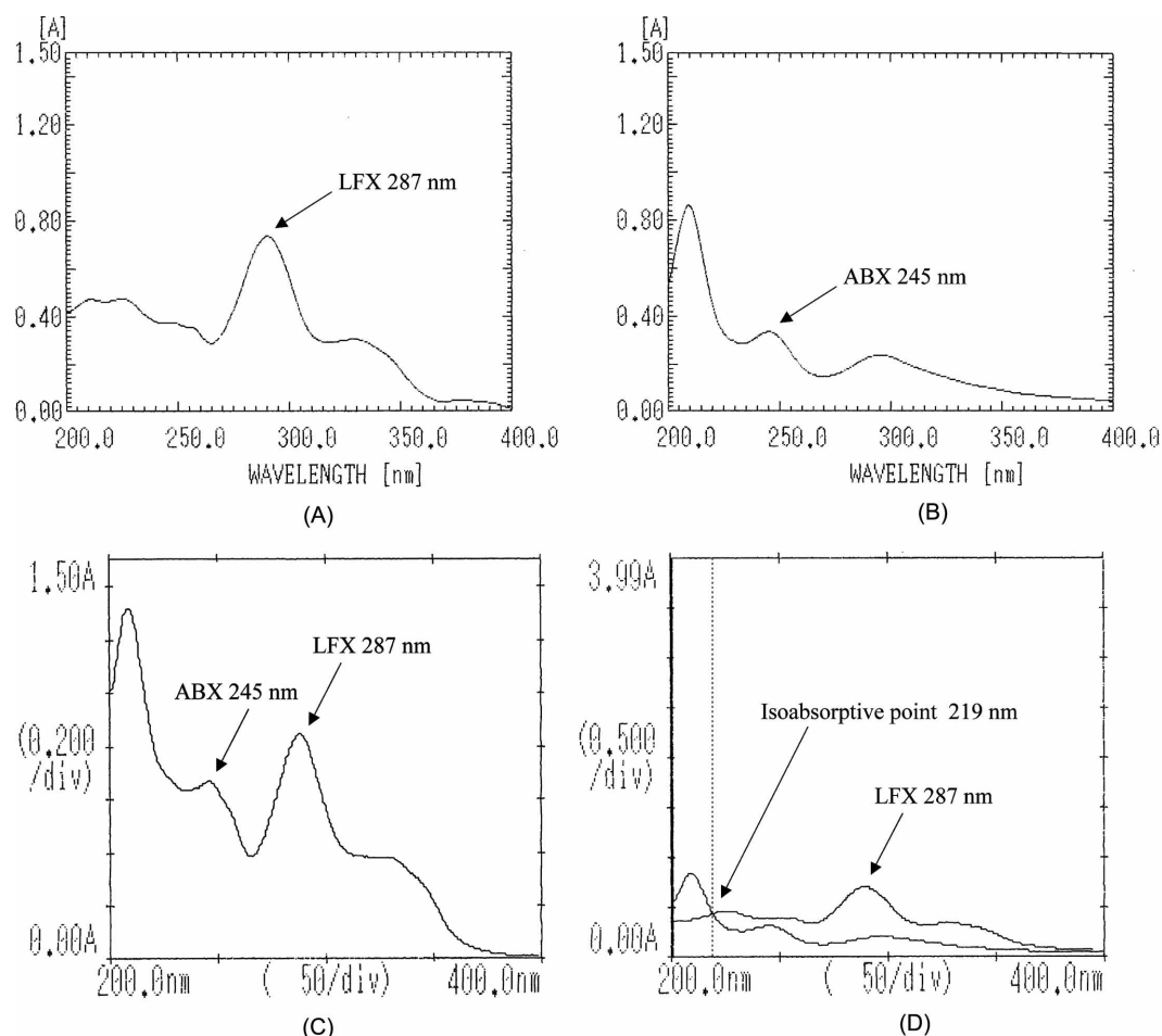
Fig. 2. (A) \lambda_{max} of levofloxacin (LFX) in distilled water, (B) \lambda_{max} of ambroxol (ABX) in distilled water. (C) \lambda_{max} of mixture of levofloxacin + ambroxol in distilled water, (D) Overlay spectra of levofloxacin and ambroxol in distilled water.
