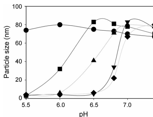
Figure 3. The particle size change ( n = 3 ) of His0 (●), His1 (■), His2 (▲), His3 (▼), His4 (◆) with pH of the solution. The micellar solution (ionic strength: 0.15) was kept to 0.1 g/L.
