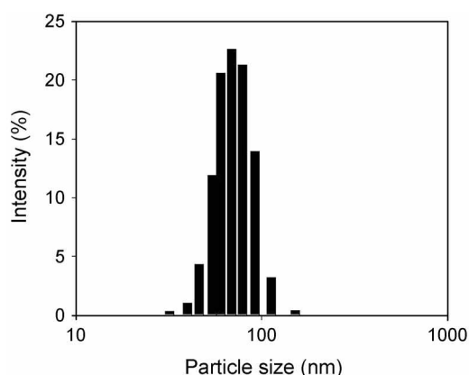
Figure 2. The particle size distribution of His1.
