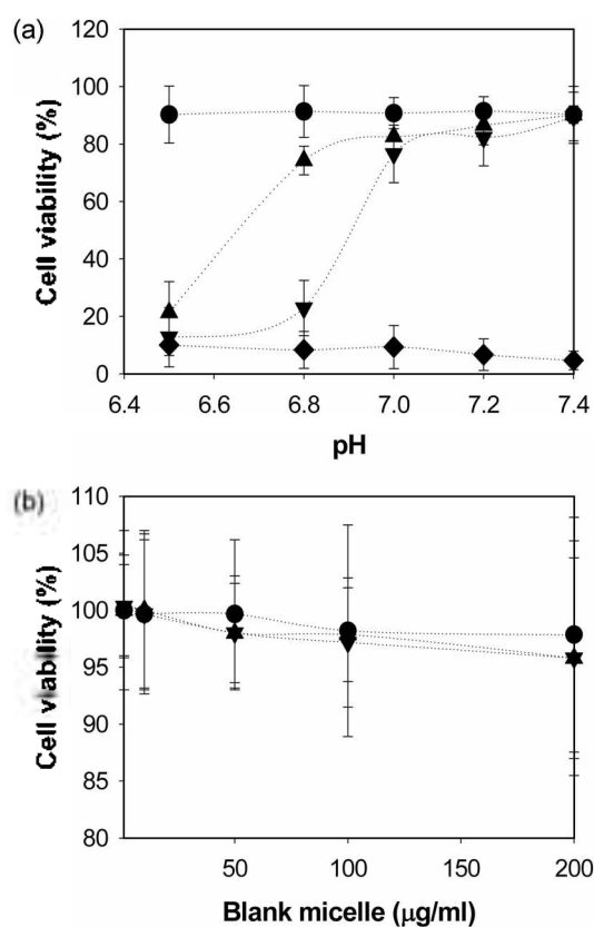
Figure 6. (a) pH-dependent MCF-7 cell viability of DOX-loaded (a) His0 (●), His2 (▲), His3 (▼) (equivalent DOX: 5 μg/mL), and free DOX (◆) (DOX: 5 μg/mL) with pH (n = 7) (b) in vitro cell toxicity of blank micelles (His0 (●), His2 (▲), and His3 (▼)) (n = 7).
