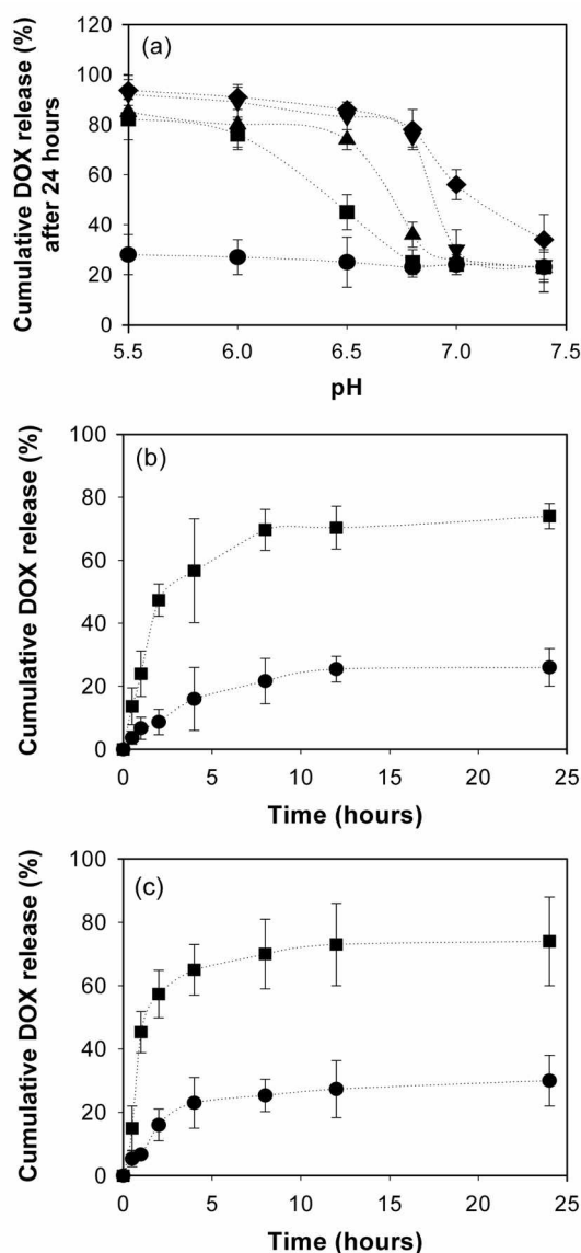
Figure 5. (a) The pH-dependent cumulative DOX release from the His0 (●), His1 (■), His2 (▲), His3 (▼), and His4 (◆) with pH ( n = 3 ) after 24 hours. The time-dependent cumulative DOX release from (b) His2 (pH 7.0: ●, pH 6.5: ■) and (c) His3 (pH 7.0: ●, pH 6.8: ■) with pH ( n = 3 ).
