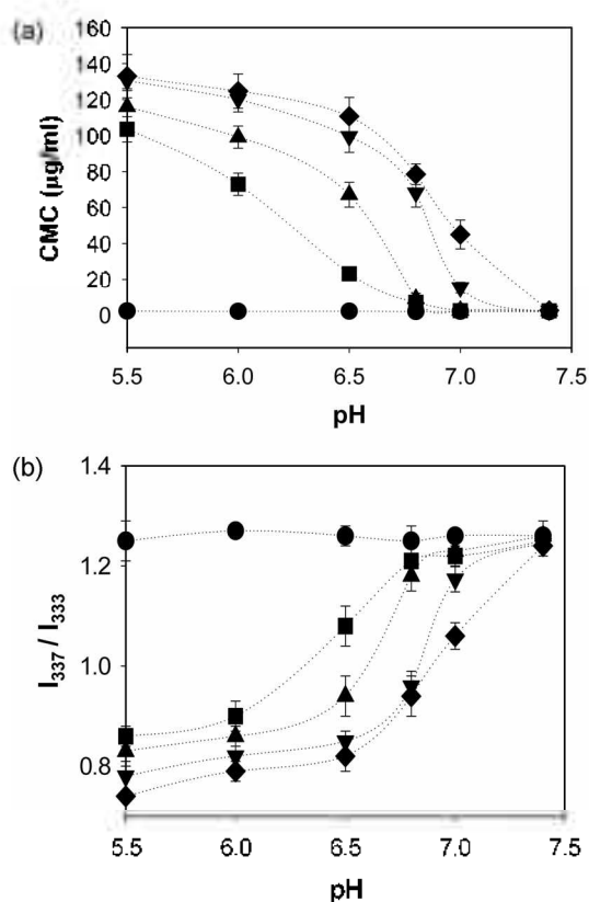
Figure 4. (a) CMC change ( n = 3 ) of His0 (●), His1 (■), His2 (▲), His3 (▼), His4 (◆) and (b) a plot of the intensity ratio I_{337}/I_{333} ( n = 3 ) of each micelle (was kept to 0.1 g/L) with pH of the solution (ionic strength: 0.15).
