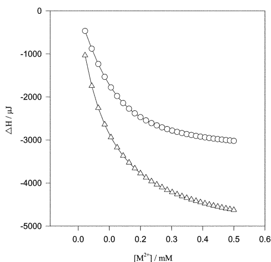
Fig. 1. The heat of Magnesium (O) and Cobalt ions (△) binding with hGH for 30 automatic cumulative injections, each of 20 \mu\text{l} , 2mM of the cations solutions, into sample cell containing 1.8 ml 35 \mu\text{M} hGH solution vs. total concentration of \text{M}^{2+} ions (Magnesium or Cobalt ions).
