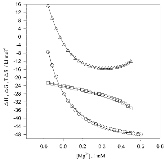
Fig. 3. Comparison between the experimental H (O), G ( ) and TS values ( ^ ) for hGH+ Mg 2+ interactions, and their calculated data (lines) via Eqs. 1 and 7. [Mg 2+ ] t is the total concentration of Mg 2+ in mM. As it is clear, the Mg 2+ -induced structural changes of hGH in the enthalpies and entropies of interactions, have canceled each other exactly in the free energies of interaction. The compensation of the structural change in the free energy is another support for Eqs. 1 and 7.
