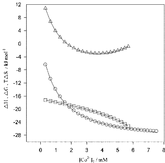
Fig. 2. Comparison between the experimental H (O), G ( ) and TS values ( ^ ) for hGH+ Co 2+ interactions, and their calculated data (lines) via Eqs. 1 and 7. [Co 2+ ] t is the total concentration of Co 2+ in mM. As it is clear, the Co 2+ -induced structural changes of hGH in the enthalpies and entropies of interactions, have canceled each other exactly in the free energies of interaction. The compensation of the structural change in the free energy is another support for Eqs. 1 and 7.
