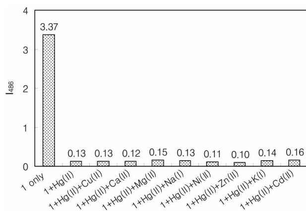
Figure 4. Changes in the fluorescence intensity of 1 at 486 nm in response to the Hg 2+ ions in the presence of various coexistent metal ions. [ 1 ] = 5.0 × 10 -6 M, [M n+ ] = 5.0 × 10 -4 M, [Hg 2+ ] = 5.0 × 10 -5 M, in aqueous acetonitrile solution (H 2 O:CH 3 CN = 50:50, v/v) buffered at pH 8.1 (10 mM of Tris). λ ex = 340 nm.
