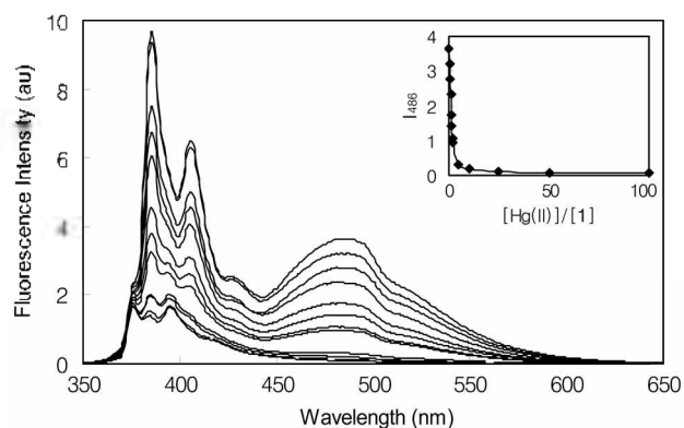
Figure 3. Fluorescence titration of 1 with \text{Hg}^{2+} ions in aqueous acetonitrile ( \text{H}_2\text{O}:\text{CH}_3\text{CN} = 50:50 , v/v). [\mathbf{1}] = 5.0 \times 10^{-6} M. \lambda_{\text{ex}} = 340 nm. In buffered solution at pH 8.1 (10 mM of Tris).
