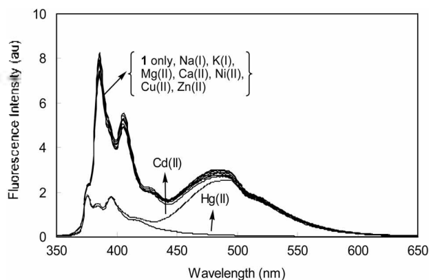
Figure 1. Fluorescence spectra of 1 in the presence of various metal ions. [\mathbf{1}] = 5.0 \times 10^{-6} M, [\text{M}^{2+}] = 5.0 \times 10^{-4} M in aqueous acetonitrile solution ( \text{H}_2\text{O}:\text{CH}_3\text{CN} = 50:50 , v/v) buffered at pH 8.1 (10 mM of Tris). \lambda_{\text{ex}} = 340 nm. The pH value denotes that of water portion before mixing with acetonitrile.
