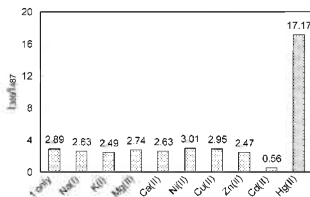
Figure 2. Changes in the fluorescence intensity ratio ( I_{386}/I_{487} ) of 1 in the presence of various metal ions. [\mathbf{1}] = 5.0 \times 10^{-6} M, [\text{M}^{2+}] = 5.0 \times 10^{-4} M in aqueous 50% acetonitrile solution buffered at pH 8.1 (10 mM of Tris). \lambda_{\text{ex}} = 340 nm.
