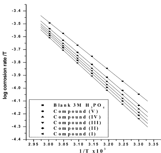
Fig. 3. log k/T 1/T curves for C-steel dissolution in 3 M H 3 PO 4 in absence and presence of 5×10 -6 M furfural hydrazone derivatives.
