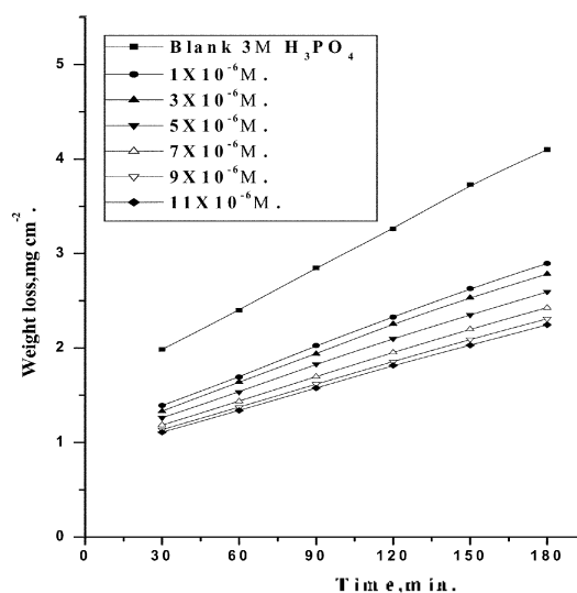
Fig. 1. Weight loss-time curves for C-steel dissolution in 3 M H 3 PO 4 in absence and presence of different concentrations of compound (1) at 30 °C.
