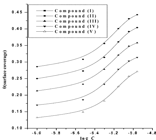
Fig. 4. θ-log C curves for C-steel dissolution in 3 M H 3 PO 4 in presence of furfural hydrazone derivatives.
