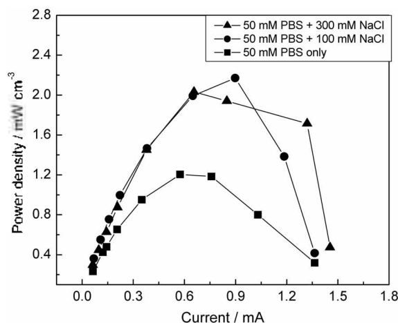
Figure 6. Polarization curves obtained for different ionic strength of NaCl: No NaCl (■), 100 mM (●), 300 mM (▲). P. vulgaris : 80 mg mL -1 . Phosphate buffer concentration was maintained at 50 mM. Other conditions are the same as Figure 2.
