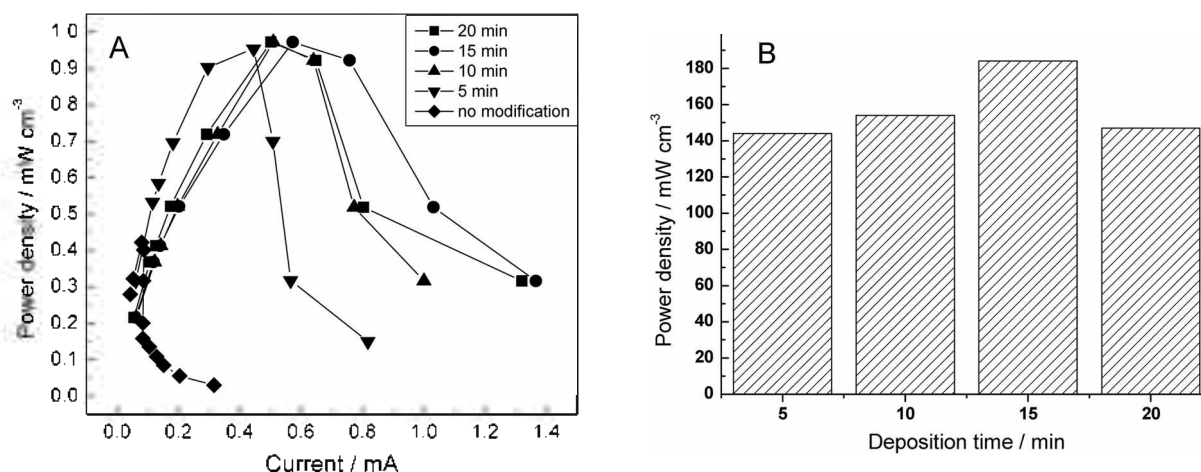
Figure 2. Polarization curves (A) and power density vs deposition time (B) for a MFC comprised of P. vulgaris (80 mg mL -1 ), methylene Blue (0.5 mM), and glucose (0.01 M) for different deposition time of 0 (◆), 5 (▼), 10 (▲), 15 (●), and 20 min (■). The solutions were buffered at pH 7.0.
