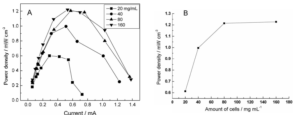
Figure 5. Polarization curves (A) obtained for different amount of bacterial cells: 20 mg mL -1 (■), 40 mg mL -1 (●), 80 mg mL -1 (▲), and 160 mg mL -1 (▼). Panel B was constructed from panel A. Other conditions are the same as Figure 2.
