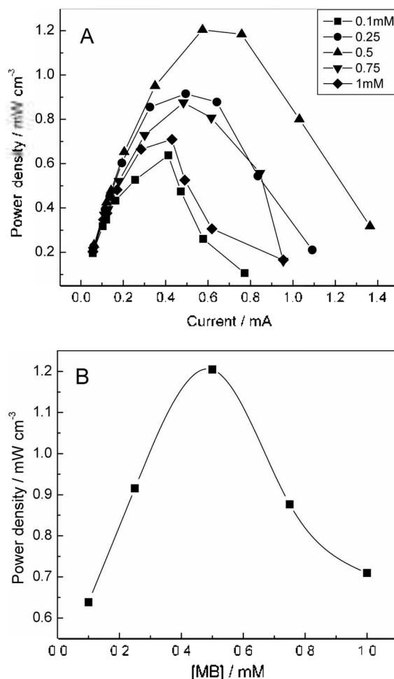
Figure 4. Polarization curves (A) and plot of power density vs methylene Blue concentration (B). MB concentration are 0.1 \text{ mM} ( \blacksquare ), 0.25 \text{ mM} ( \bullet ), 0.5 \text{ mM} ( \blacktriangle ), 0.75 \text{ mM} ( \blacktriangledown ), and 1 \text{ mM} ( \blacklozenge ). Other conditions are the same as Fig. 2. Electrodeposition time was 15 min.
