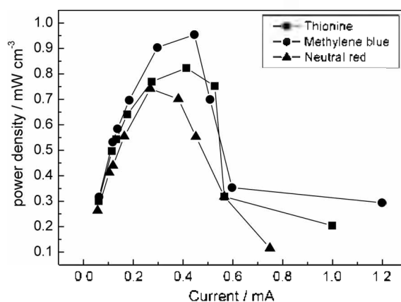
Figure 3. Polarization curves obtained when different mediators were used. Other conditions are the same as Fig. 2. Mediators ( 0.5 \text{ mM} ) are thionin ( \blacksquare ), methylene Blue ( \bullet ), and neutral Red ( \blacktriangle ). Electrodeposition time was 5 min.
