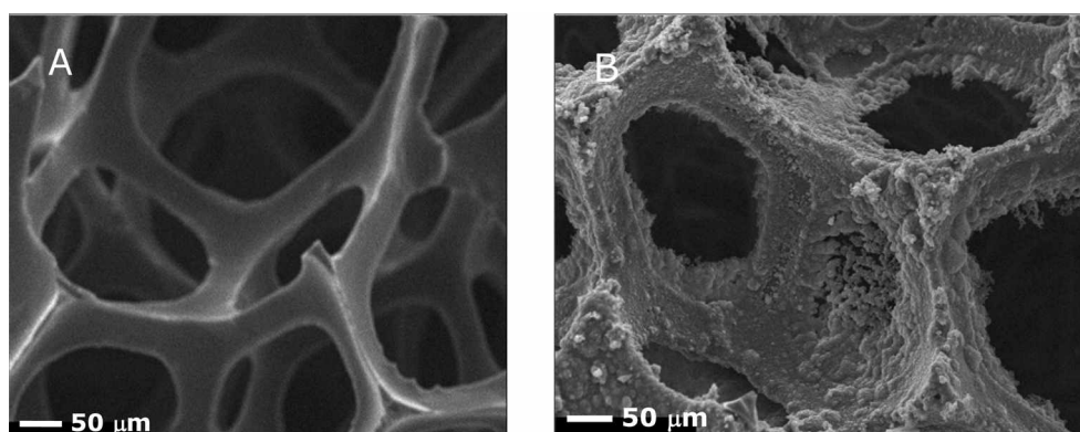
Figure 1. SEM images of RVC before (A) and after (B) electropolymerization of pyrrole for 15 min.
