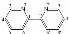
Figure 1. Chemical structure of 2,2-bipyridine with atomic numbering.
