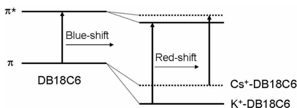
Figure 5. Schematic energy diagram illustrating the red-shift of the S_1 band of \text{Cs}^+ -DB18C6 from that of \text{K}^+ -DB18C6.
