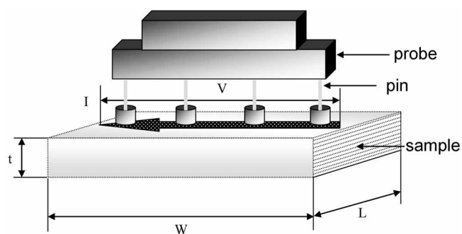
Figure 2. Schematic diagram of specific resistivity measurement.
