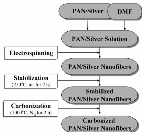
Figure 1. Sampling process for electrospun PAN/silver-based carbon nanofibers.
