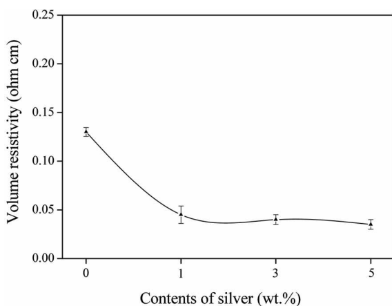
Figure 6. Volume resistivity of PAN/silver-based carbon nanofibers with different silver contents.
