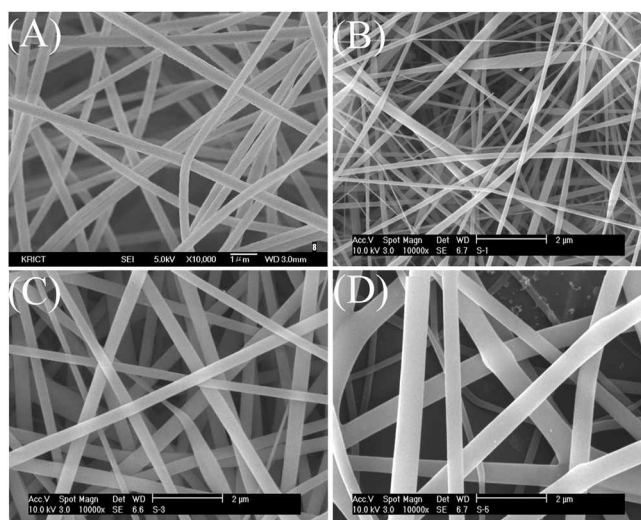
Figure 3. SEM images of PAN/silver-based nanofiber webs with silver contents ranging from (A) 0 wt.%, to (B) 1 wt.%, (C) 3 wt.%, and (D) 5 wt.%.
