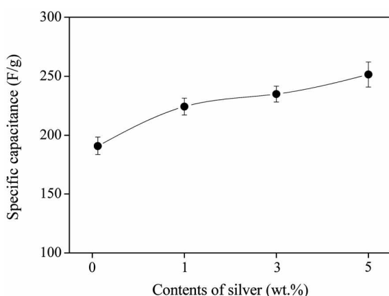
Figure 5. Specific capacitance of PAN/silver-based nanofibers with different silver contents.
