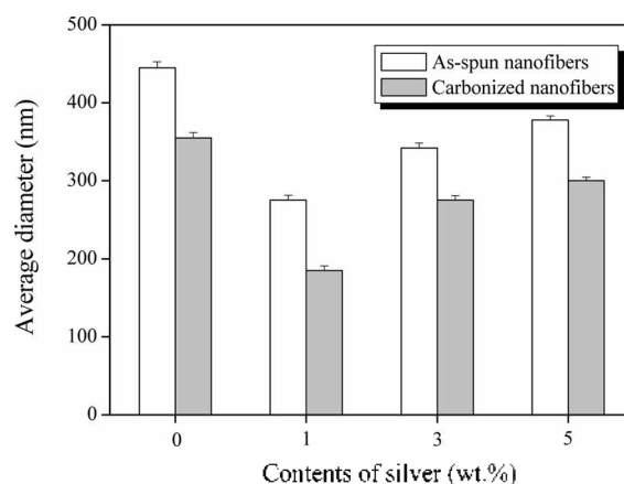
Figure 4. Diameter distribution of PAN/silver-based carbon nanofibers before and after carbonization process with different silver contents.
