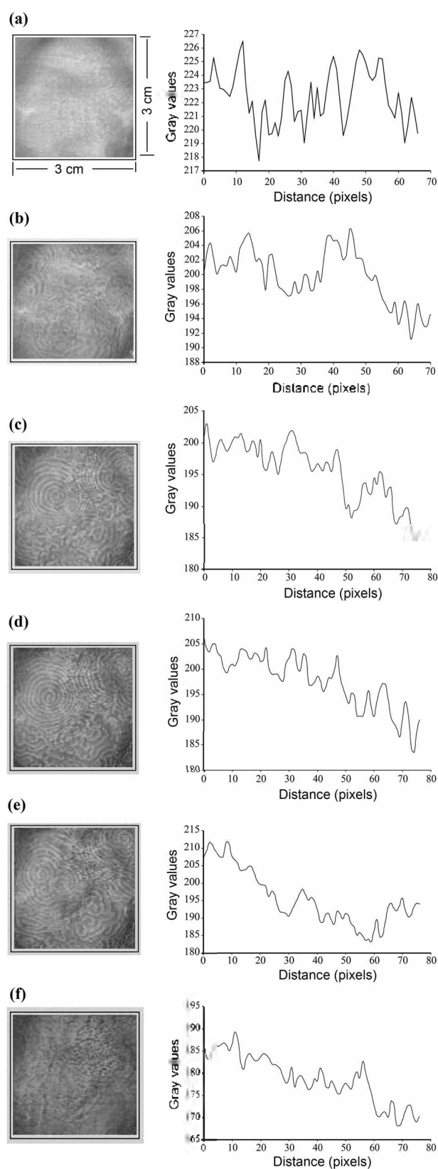
Figure 1. Typical propagating waves with a spiral pattern obtained in a micro-emulsion medium at [\text{BrO}_3^-]_0 = 0.6\text{M} , [\text{1,4-CHD}]_0 = 0.12 , [\text{ferroin}]_0 = 0.49 mM, and [\text{H}^+]_0 = 0.3 M; and at t = (a) 30, (b) 60, (c) 115, (d) 130, (e) 136, and (f) 170 min. The figures in the right-hand side of the wave patterns show their plot profiles in each time.
