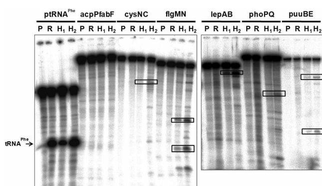
Figure 2. RNase P cleavage reaction. Model substrate RNAs for each polycistronic mRNA were prepared by in vitro transcription. The \text{ptRNA}^{\text{Phe}} (100 nM) and model substrate RNAs (50 nM) labeled at the 5' ends were incubated with RNase P for 40 min at 37 °C. The acpPfabF model RNA (323 nt), cysNC model RNA (287 nt), flgMN model RNA (264 nt), lepAB model RNA (210 nt), phoPQ model RNA (300 nt), and puuBE model RNA (292 nt), were used. Lane P, C5 protein 200 nM; Lane R, MI RNA 55 nM; Lane H 1 , RNase P holoenzyme 2 nM; Lane H 2 , RNase P holoenzyme 20 nM. Reaction products were separated on an 8% (w/v) polyacrylamide gel containing 7 M urea. The cleavage products of model substrate RNAs by RNase P holoenzyme are indicated in boxes.
