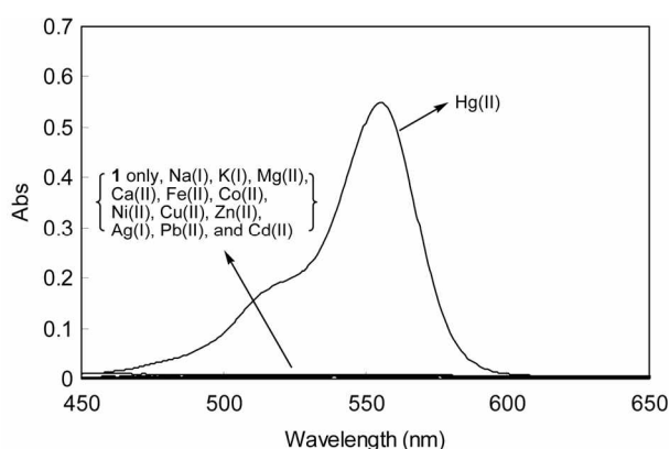
Figure 1. UV-Vis spectra of 1 in the presence of various metal ions in an aqueous methanol solution at pH 5. [ 1 ] = 5.0 \times 10^{-6} M, [ M^{n+} ] = 5.0 \times 10^{-4} M, in H_2O - CH_3OH (90:10, v/v) at pH 5.0 (acetate buffer, 10 mM). The indicated pH value denotes the pH of the H_2O portion before adding methanol.
