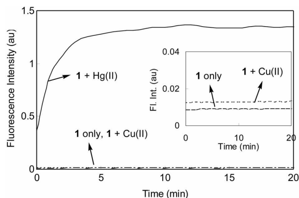
Figure 4. Fluorescence intensity of 1 at 578 nm as a function of time in the presence of \text{Hg}^{2+} and \text{Cu}^{2+} ions. [1] = 5.0 \times 10^{-6} M, [\text{M}^{2+}] = 5.0 \times 10^{-4} M, in \text{H}_2\text{O}-\text{CH}_3\text{OH} (90:10, v/v) at pH 5.0. \lambda_{\text{ex}} = 500 nm.
