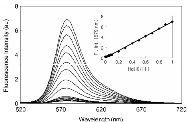
Figure 3. Fluorescence spectra of 1 as a function of concentration of \text{Hg}^{2+} ions. [1] = 2.0 \times 10^{-5} M in \text{H}_2\text{O}-\text{CH}_3\text{OH} (90:10, v/v) at pH 5.0. \lambda_{\text{ex}} = 500 nm.
