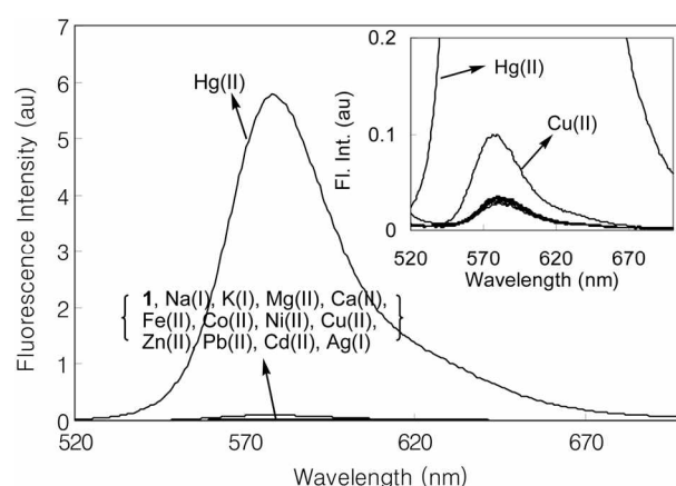
Figure 2. Fluorescence spectra of 1 in the presence of various metal ions. [ 1 ] = 5.0 \times 10^{-6} M, [ M^{n+} ] = 5.0 \times 10^{-4} M, in buffered H_2O - CH_3OH (90:10, v/v) at pH 5.0. \lambda_{ex} = 500 nm.
