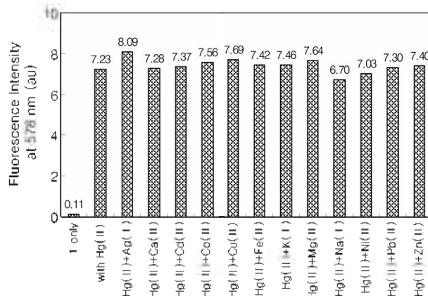
Figure 5. Selective signaling of \text{Hg}^{2+} ions by 1 in the presence of common interfering metal ions. [1] = 5.0 \times 10^{-6} M, [\text{Hg}^{2+}] = 5.0 \times 10^{-5} M, [\text{M}^{2+}] = 5.0 \times 10^{-4} M, in buffered \text{H}_2\text{O}-\text{CH}_3\text{OH} (90:10, v/v) at pH 5.0. \lambda_{\text{ex}} = 500 nm.
