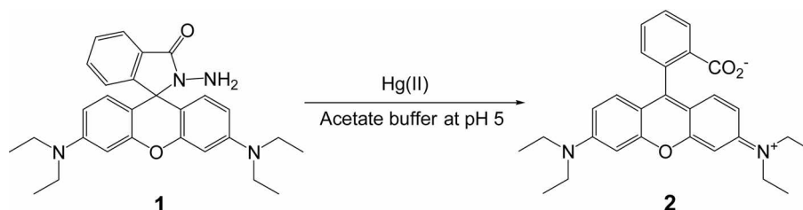
Scheme 2. Hg^{2+} -selective signaling of hydrazide 1 .
