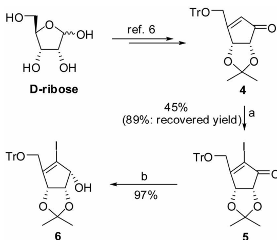
Scheme 2. (a) \text{I}_2 , pyridine, \text{CCl}_4 , rt, 12 h; (b) \text{NaBH}_4 , \text{CeCl}_3 \cdot 7\text{H}_2\text{O} , \text{MeOH} , 0^\circ\text{C} , 30 min.
