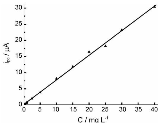
Figure 7. Calibration curve for artemisinin. Accumulation time: 3 min.
