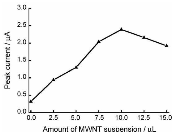
Figure 5. Effect of amount of MWNT/DHP suspension on the reduction peak current of 3.0 \text{ mg L}^{-1} artemisinin. Accumulation time: 3 min.
