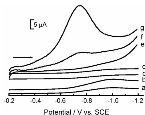
Figure 4. LS voltammograms of 30.0 \text{ mg L}^{-1} artemisinin in pH 7.0 phosphate buffer at GCE (a,b), DHP-modified GCE (c,d) and MWNT/DHP modified GCE (f,g). (b,d,g): after 3-min accumulation; (e): blank voltammograms of MWNT/DHP film. Scan rate: 100 \text{ mV s}^{-1} .
