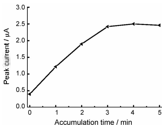
Figure 6. Influence of accumulation time on the reduction peak current of 3.0 \text{ mg L}^{-1} artemisinin.
